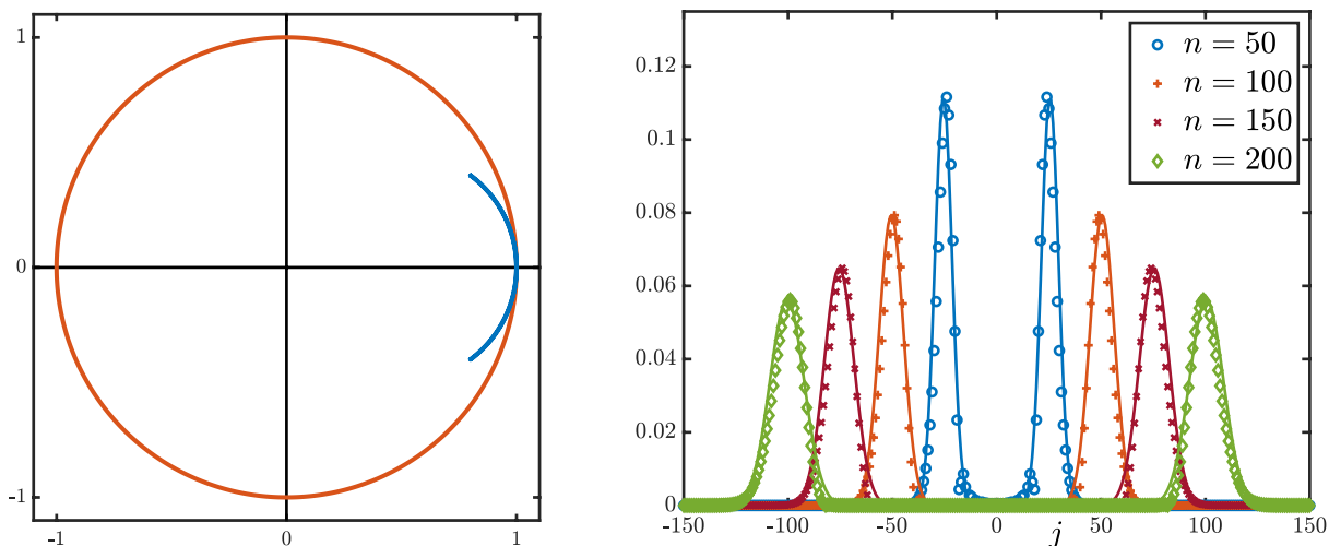
Figure 8: Left: Spectrum (blue curve) \sigma(\mathcal{L}) = F(\mathbb{S}^1) for the implicit scheme (42) with \lambda = 1/2 . Right: The absolute value of the Green's function (marked points) at different time iterations for the implicit scheme (42) compared with two fixed Gaussian profiles centered at j = \lambda n and j = -\lambda n (solid lines). We started with an initial condition given by the Dirac mass \delta .
