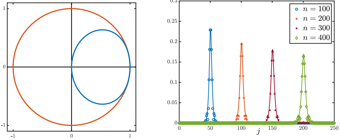
Figure 9: Left: Spectrum (blue curve) \sigma(\mathcal{L}) = F(\mathbb{S}^1) for the O3 scheme (43) with \lambda = 1/2 . Right: The absolute value of the Green's function (marked points) at different time iterations for the O3 scheme (43) compared with a fixed generalized Gaussian profile \mathcal{H}_j^n (44) centered at j = \lambda n (solide lines). We started with an initial condition given by the Dirac mass \delta .
