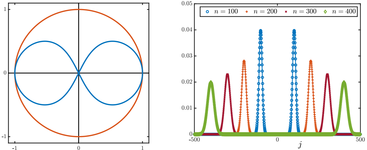
Figure 11: Left: Spectrum (blue curve) \sigma(\mathcal{L}) = F(\mathbb{S}^1) for the \infty scheme (45). Right: The absolute value of the Green's function (marked points) at different time iterations for the \infty scheme (45) compared with two fixed Gaussian profiles centered at j = n and j = -n (solid lines). We started with an initial condition given by the Dirac mass \delta .
