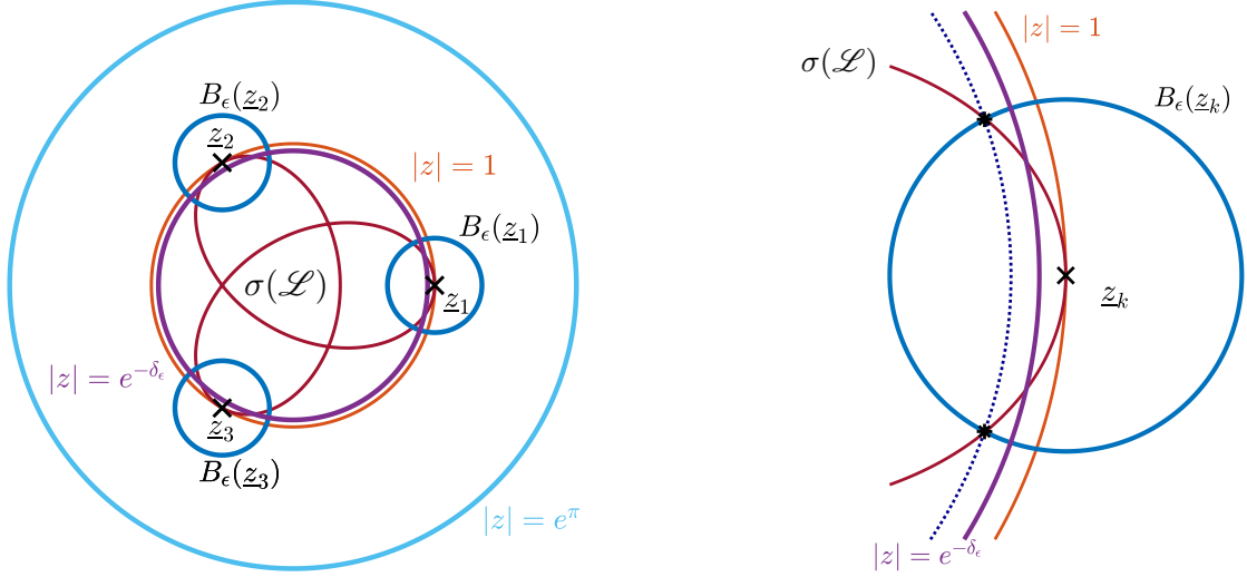
Figure 1: Geometrical illustrations of the set \mathcal{S} given in Corollary 1 in the case K = 3 . The curve of essential spectrum \sigma(\mathcal{L}) (dark red curve) is tangent to the unit circle precisely at z_k for k = 1, 2, 3 (black crosses) and otherwise strictly contained in the unit disk \mathbb{D} . For \epsilon \in (0, \epsilon_*) , each ball B_\epsilon(z_k) intersects \sigma(\mathcal{L}) at two points (black stars in the right panel) and the dashed dark blue line represents the circle passing through the point with largest modulus. We then fix \delta_\epsilon > 0 such that the circle \{z \mid |z| = e^{-\delta_\epsilon}\} (magenta curve) is contained in between the unit circle and the circle passing through the point with largest modulus.
