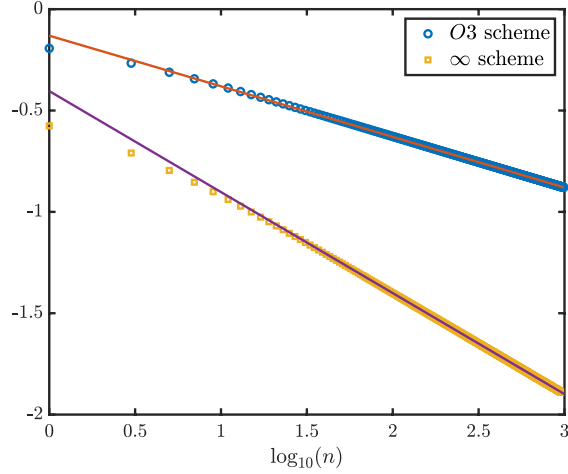
Figure 10: Illustration of the scaling factor in the generalized Gaussian bounds provided by Theorem 1 in the case of the O3 scheme (blue circles) and the \infty scheme (orange squares). We plot \log_{10} \left( \sup_{j \in \mathbb{Z}} |\mathcal{G}_j^n| \right) as a function of \log_{10}(n) together with a best linear fit for each scheme for n ranging from 1 to 10^3 . For the O3 scheme we find a slope of -0.2496 while for the \infty scheme we find a slope of -0.4983 which compare well with the theoretical -1/4 and -1/2 scaling factors.
