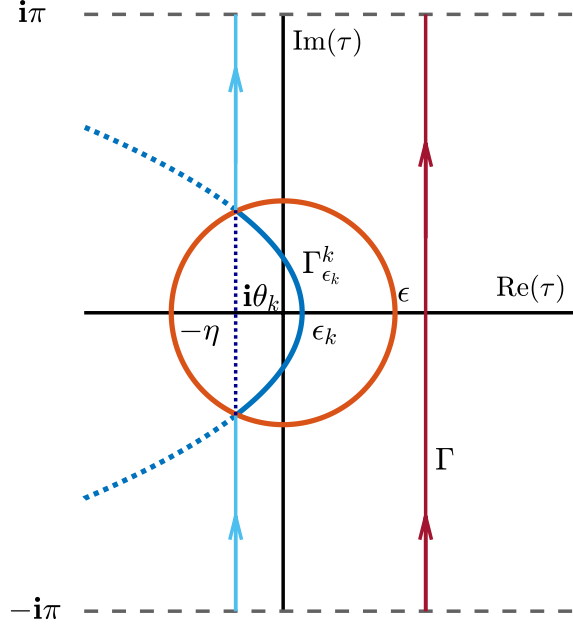
Figure 6: Illustration of the contour \Gamma_{\epsilon_k}^k used in the proof of Lemma 14 and Lemma 15.
