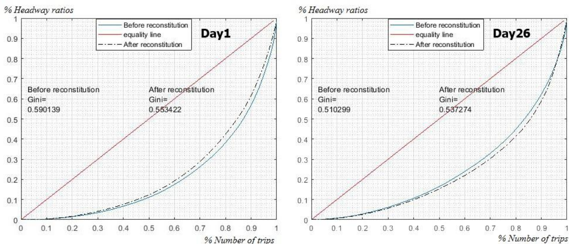
Fig. 5. Lorenz curve for all the stops before and after data reconstitution
