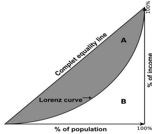
Fig. 1. The Lorenz curve
