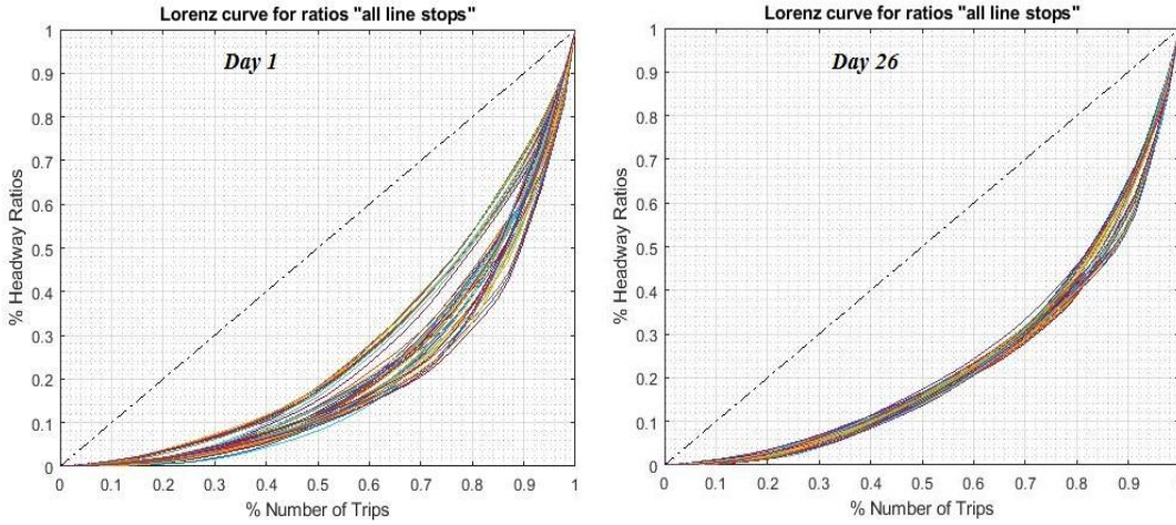
Fig. 6. Lorenz curves for all 53 stops separately (day1 and day 26)
