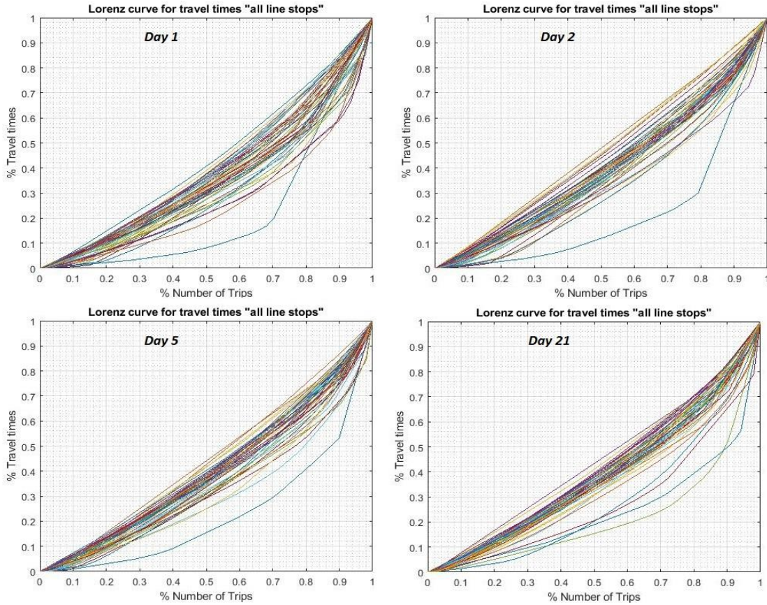
Fig. 7. Lorenz curves drawn for travel times for several days
