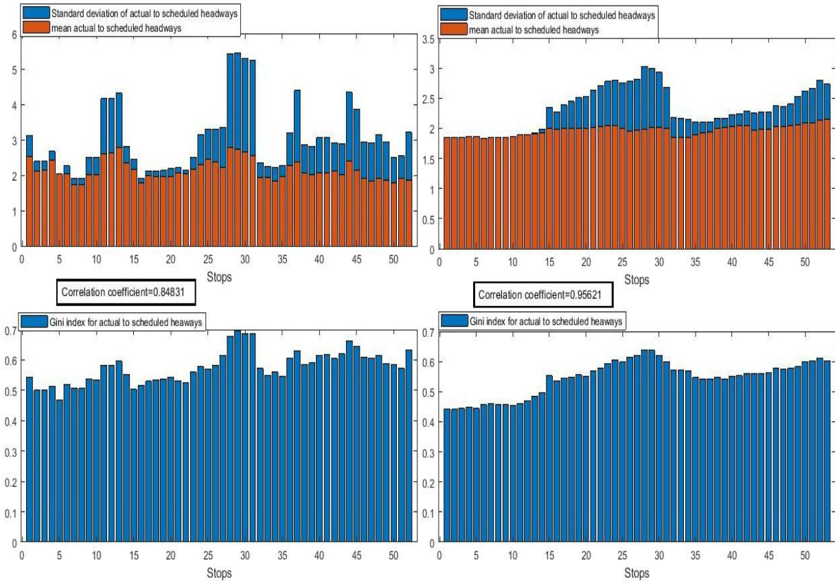
Fig. 4. Correlation before (left)
