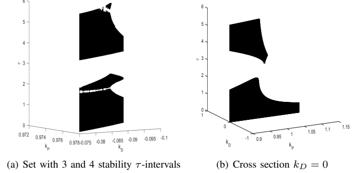
Fig. 11. Stability set for Example 10
