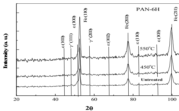
Fig. 2 Bragg-Brentano mode of X-ray diffraction profiles of as-received and nitrided CrMoV steels at variable temperatures (450 and 550 °C) for a fixed duration of 6h.
