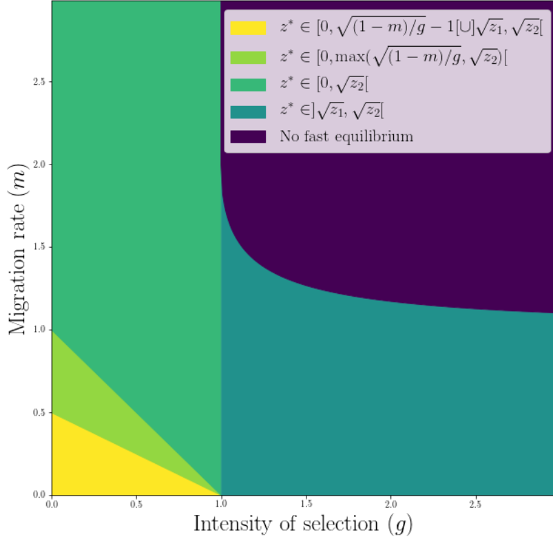
Figure 3: Description of the conditions imposed on z^* \geq 0 to get a fast equilibrium depending on the pair (g, m) under the preliminary assumption that P_{z^*} has a single positive root, according to the results of Proposition 3.1 . When selection is smaller than 1, symmetrical fast equilibria exist ( z^* = 0 ), and do not when selection is larger than 1. When both migration and selection are both too strong, no fast equilibrium can exist.
