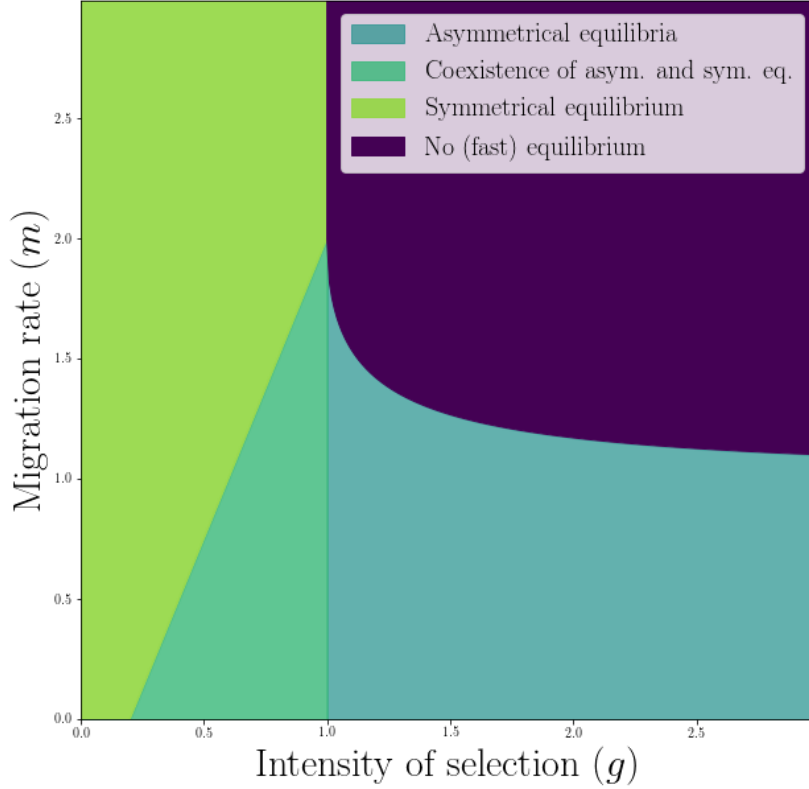
Figure 4: Regions of existence of the equilibria, according to Proposition 4.1 and Proposition 4.2 . The symmetrical equilibrium is only determined by the intensity of selection, regardless of the migration rate. The asymmetrical equilibria cannot exist for large migration rate ( m > 2 ) or small intensity of selection. The limit of the blue region is given by m = 1 when g goes to \infty . Interestingly enough, at intermediate migration: m \in [1, 2] , asymmetrical equilibria only exist for a bounded range of positive g : selection cannot be too strong nor too weak. Moreover, see Section 4.2 for stability results about these equilibria to determine which equilibria prevail when both symmetrical and asymmetrical coexist (turquoise triangular region).
