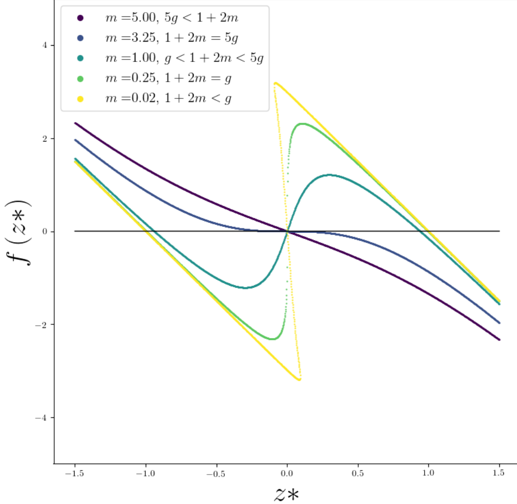
Figure 5: Graph of the function f for g = 1.5 and m \in \{0.02, 0.25, 1, 3.25, 5\} . The dominant traits z^* of the different equilibria are located where the curve crosses the horizontal line ( f(z^*) = 0 ). An equilibrium is locally stable if the slope of f at the point of equilibrium is negative. For decreasing values of m (dark to light colors), at first, only the symmetric equilibrium exists and is stable (see also Corollary 2 ). Then, the asymmetrical equilibria emerge (in the parameter region indicated in Proposition 4.2 ) and are bistable (see also Corollary 3 ), while the symmetric equilibrium becomes unstable. For small values of m , the curve folds near the origin, as for z^* near 0, P_{z^*} has three distinct positive roots ( Proposition 3.2 ). For those z^* , the fast equilibria are all non viable ( Lemma 2 ): numerically, the system goes to extinction if the initial dominant trait is near 0.
