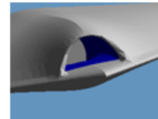
group 4 : Intake-tube T_{avg,4} = 282 \text{ K} \epsilon_4 = 0,9 Lambertian
