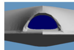
group 8 : Disc at intake end T_{avg,8} = 284 \text{ K} \epsilon_8 = 0,92 Lambertian
