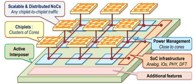
Fig. 3. Active Interposer concept and main features
