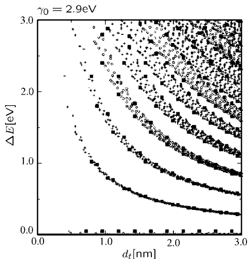
FIG. 30. Energy separation E_{ii}(d) for all (n, m) values as a function of CNT diameter d_t , with 0.7 \leq d_t \leq 3.0 nm. Crosses and open circles denote the peaks of semiconducting and metallic tubes, respectively. Solid squares denote E_{ii}(d) values for zigzag tubes. Adapted from Saito, Dresselhaus, and Dresselhaus, 2000.
