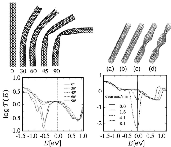
FIG. 46. Transmission coefficient as a function of Fermi level for isolated bent (6,6) nanotubes with increasing bending angle (left) or for twisted models of distortions (right). Upper drawings show the corresponding nanotube structures. Adapted from Rochefort et al. , 1999.
