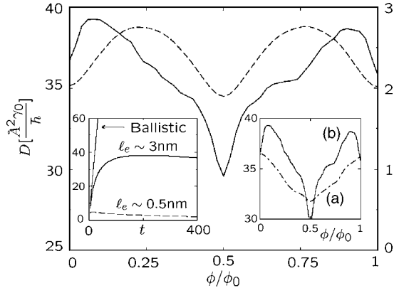
FIG. 47. Diffusion coefficient \mathcal{D}(\tau_\phi, \phi/\phi_0) (in units of \text{\AA}^2\gamma_0/\hbar ) for the (9,0) nanotube evaluated at time \tau_\phi \gg \tau_e for two disorder strengths W/\gamma_0=3 and 1 such that the mean free path ( \ell_e \sim 0.5 and 3 nm, respectively) is either shorter (dashed line) or longer (solid line) than the nanotube circumference ( |C_h| \sim 2.3 nm). The right y axis is for the dashed line, and the left y axis is for the solid line. Inset: \mathcal{D}(\tau_\phi, \phi/\phi_0) for \ell_e=3 nm and L(\tau_\phi) < 2\ell_e .
