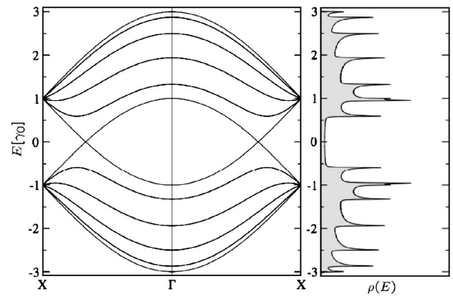
FIG. 10. Band structure and density of states for a (5, 5) armchair nanotube within the zone-folding model. The 1D energy dispersion relations are presented in the [-3\gamma_0; 3\gamma_0] energy interval in dimensionless units ( \gamma_0 being the nearest-neighbor C-C tight-binding overlap energy \sim 2.9 eV). The energy bands are plotted along the X - \Gamma - X direction. The Fermi level is located at zero energy.
