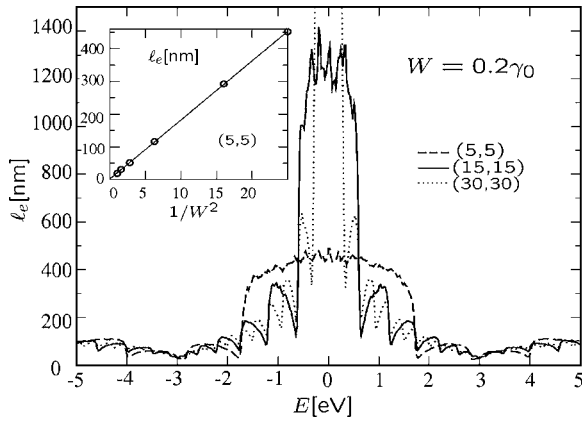
FIG. 38. Energy-dependent mean free path as a function of diameter. Inset: 1/W^2 scaling in agreement with the Fermi golden rule. Adapted from Trioizon et al., 2004 .
