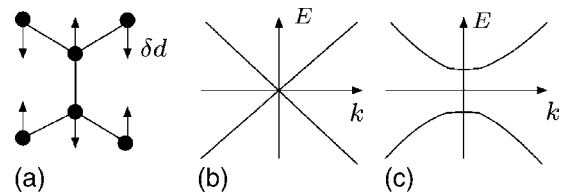
FIG. 51. Band gap opening by optical phonons. (a) Displacement pattern of the longitudinal (transverse) A_1 mode in a zigzag (armchair) tube. Band structure for a metallic zigzag tube in (b) the equilibrium positions and (c) for the distortion compatible with the A_1(L) mode. Adapted from Dubay et al. , 2002.
