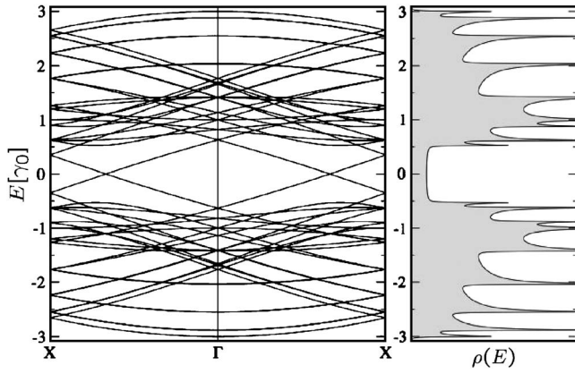
FIG. 13. Band structure and density of states for a (8,2) chiral nanotube within the zone-folding model. The Fermi level is located at zero energy.
