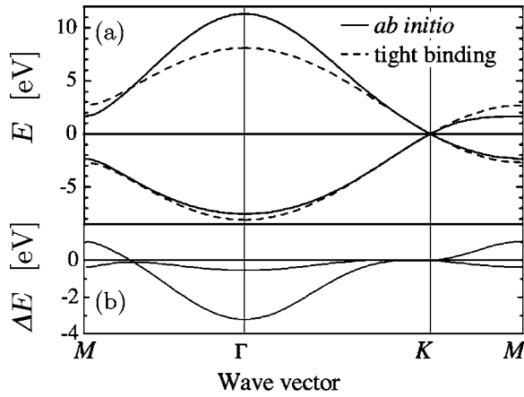
FIG. 7. Limitations of the \pi - \pi^* model. (a) Ab initio (solid lines) and nearest-neighbor orthogonal tight-binding [dashed lines, from Eq. (14)] \pi and \pi^* electronic bands for graphene. (b) Difference \Delta E between the ab initio and tight-binding band structures. Adapted from Reich, Maultzsch, Thomsen, and Ordejón, 2002.
