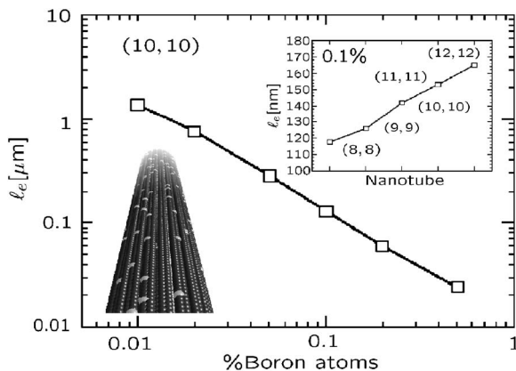
FIG. 41. Scaling of the mean free path at the Fermi level, for a B-doped ( n,n ) nanotube. Left: In the case of a (10,10) nanotube with various boron concentrations, \ell_e behaves like the inverse of the doping rate. Right: For a fixed concentration of B atoms, \ell_e is a linear function of the nanotube's diameter.
