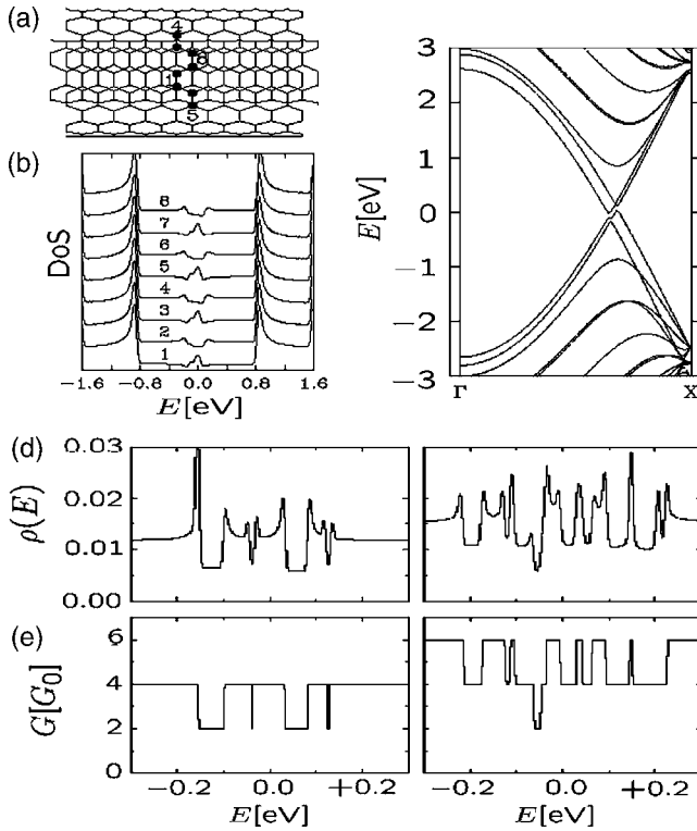
FIG. 42. Effect of the rotational symmetry breaking for a commensurate (5,5)@(10,10)@(15,15) MWNT on (a) its electronic properties, (b) its DOS, and (c) its band structure. Adapted from Lambin et al., 2000 . Pseudogaps (d) and associated conductance spectra (e) for (5,5)@(10,10)@(15,15). Adapted from Sanvito et al., 2000 .
