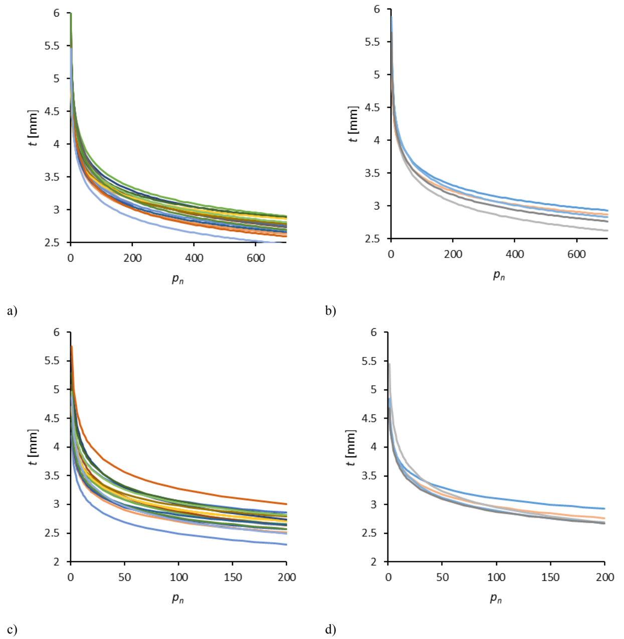
Figure 9. Fitted wet compaction curve for [thickness measurement source - material] a) [UTM - NCF wet], b) [LVDT/direct - NCF wet], c) [UTM - WOVEN wet] and d) [LVDT/direct - WOVEN wet].
