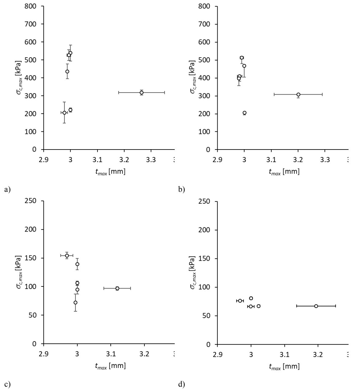
Figure 6. Maximum compaction stress, \sigma_{c,max} , and corresponding measured thickness, t_{max} , obtained with LVDT or other direct thickness measurement for a) NCF dry, b) WOVEN wet, c) NCF dry and d) WOVEN wet.
