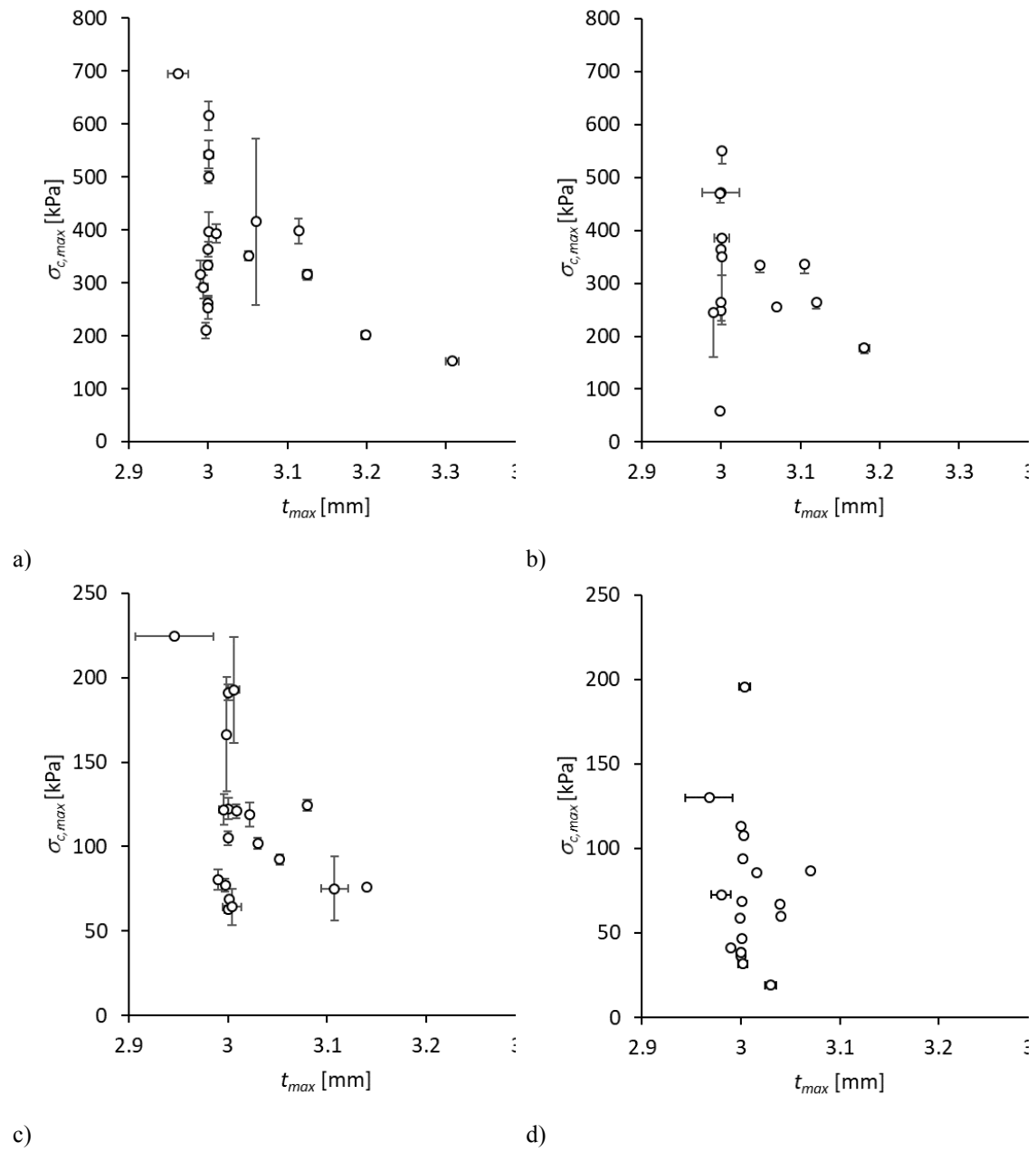
Figure 5. Maximum compaction stress, \sigma_{c,max} , and corresponding measured thickness, t_{max} , obtained with UTM thickness measurement for a) NCF dry, b) NCF wet, c) WOVEN dry and d) WOVEN wet.
