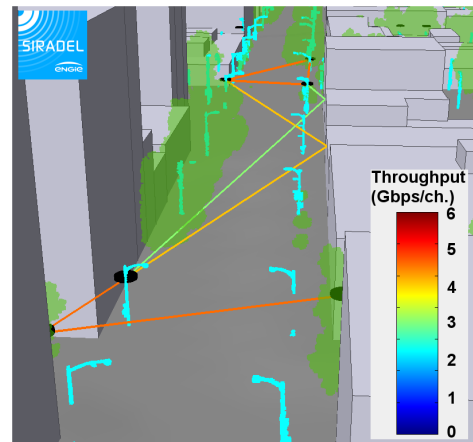
Figure 3: Direct and indirect connections.
