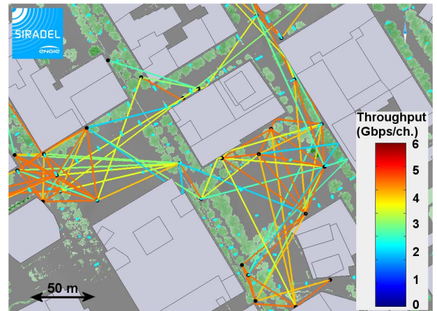
Figure 2: Mesh links in the outdoor backhaul network.
