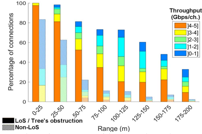
Figure 4: Percentage of links reaching a given throughput vs. distance.
