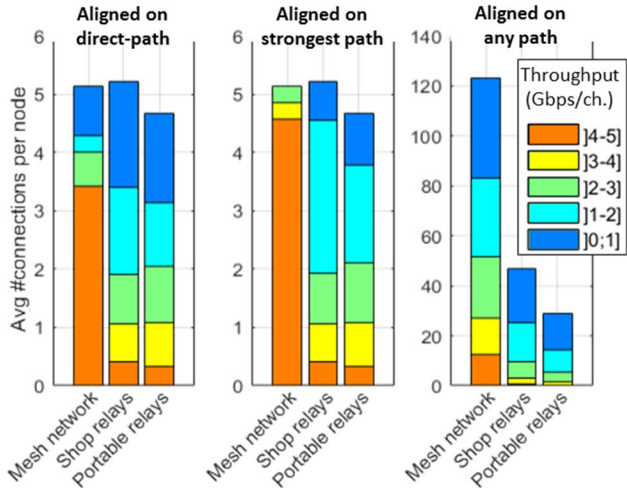
Figure 7: Number of connections per throughput range.
