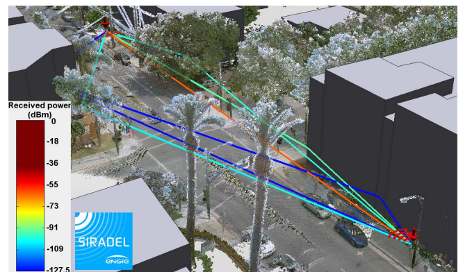
Figure 1: Propagation path within LiDAR data.
