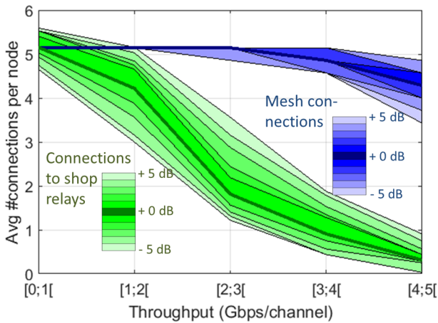
Figure 8: Number of connections per throughput range vs. link budget adjustment.
