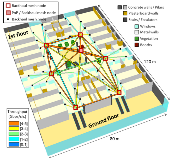
Figure 6: Main connections between mesh nodes, and to the shop-relays.
