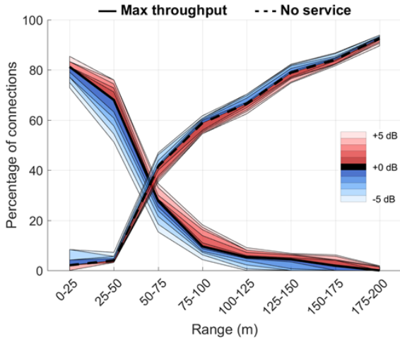
Figure 5: Percentage of links reaching max. throughput, or without any connection, vs. link budget gain.
