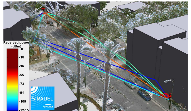
Figure 1: Propagation path within LiDAR data.
