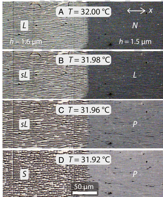
Q:14 Fig. 3. Textures observed across a step of thickness upon cooling an 8CB film with intermediate ( 1.5 \mu\text{m} < h < 2.0 \mu\text{m} ) and small ( h \leq 1.5 \mu\text{m} ) thickness. P is a texture with smooth and straight stripes perpendicular to the planar anchoring direction x .
