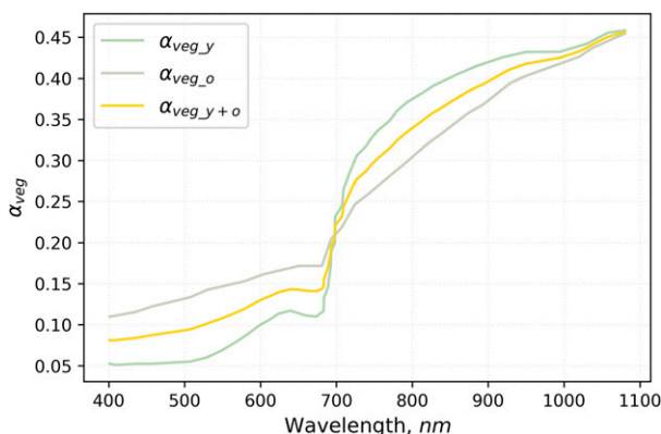
FIG. A2. Branch reflectivity measured by Juszak et al. (2014) for young branches ( \alpha_{veg\_y} ), old branches ( \alpha_{veg\_o} ) and the average of old and young branches ( \alpha_{veg\_y+o} ). Figure adapted from Belke-Brea et al. (2019).
