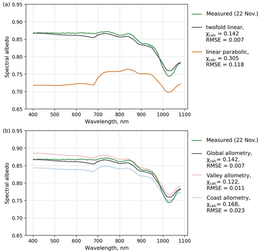
FIG. 6. Example highlighting model sensitivity to the choice of exposed-vegetation function and allometric equation. Measured albedo, taken on 22 Nov in the valley near Umiujaq, is shown together with (a) two spectra simulated with different exposed-vegetation functions and (b) three spectra simulated with different allometric equations. All simulated spectra in (b) were calculated using the twofold approach [shown in Eqs. (8) and (9)]. The best fit between measured and modeled data was achieved by using the twofold approach together with global allometry (gray curve).
