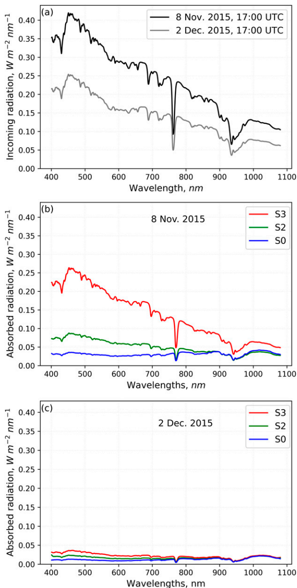
FIG. 10. Spectral incoming radiation as calculated with SBDART and the corresponding spectra of absorbed radiation at the lichen site S0 (blue), medium shrub site S2 (green), and tall shrub site S3 (red). (a) Incoming radiation for 8 Nov and 2 Dec at 1700 UTC for overcast conditions. Spectra of absorbed radiation for 8 Nov are shown in (b) and those for 2 Dec in (c).
