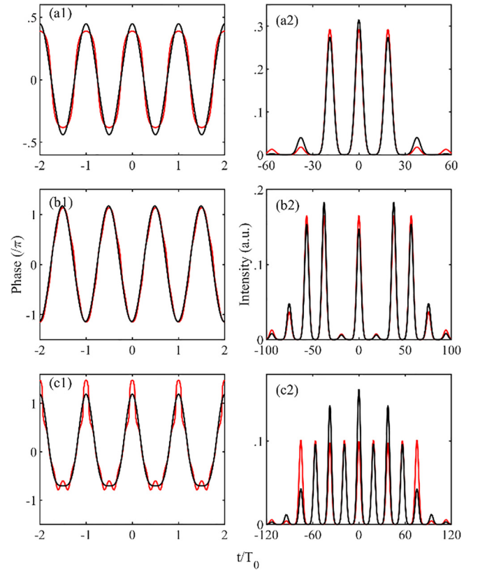
Fig. 6. Comparison between the output waveforms (panels 2) modulated with ideal phase profiles and BW-limited ones depicted in panels 1 (red and black lines, respectively) for N = 3, 7 and 9 peaks (panels (a), (b) and (c), respectively). BW limitation assumed to be of a super-Gaussian of order 4 with a width of 4f_m . (For interpretation of the references to colour in this figure legend, the reader is referred to the web version of this article.)
