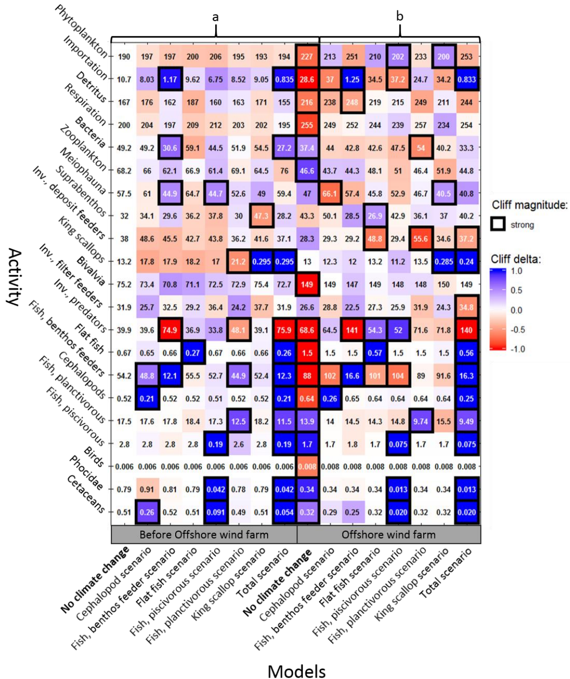
357 Figure 6: Variation of all the throughflow/activity (input/output) in gC.m 2 between: the BOWF model 358 and the single effect models (reef effect or climate change effect, a group on the left), and between 359 the REEF model and the cumulative models (reef effect + climate change effect, b group on the 360 right). Red, increased activity; blue, decreased activity; bold-bordered square, strong variation 361 according to the cliff delta ( |\partial \text{Cliff}| < 0.474 ).
