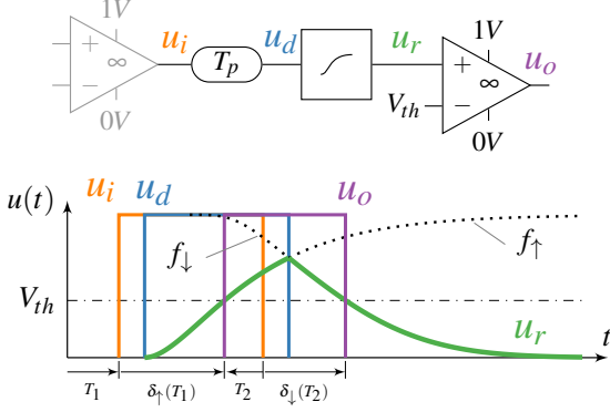
Figure 3: Simple analog channel model (upper part) with a sample execution (bottom part) taken from [10]. At a transition on u_d (blue) the transitions waveforms are immediately switched (green).
