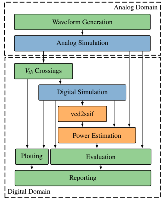
Figure 6: Workflow in the invTool . The green parts had to be implemented from scratch. The blue parts have been available, albeit the available resources had to be extended significantly. Orange parts could be used almost out of the box.
