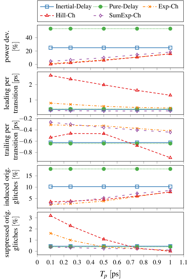
Figure 13: MIPS clock circuit simulation results (15 nm) for \mu = 15 ps.
