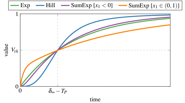
Figure 4: Sample switching waveforms for the utilized IM channels (only one direction shown). Recall that the SumExp-channel provides more degrees of freedom than the other ones.
