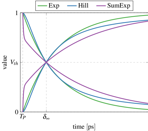
(a) switching waveforms
