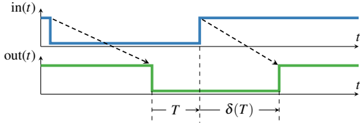
Figure 1: Principle functionality of a single-history delay model. Based on the input-to-previous output transition time T , the delay \delta(T) is determined.
