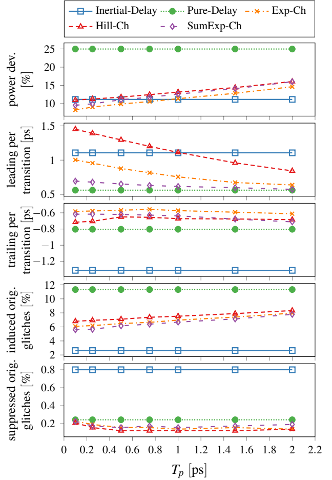
Figure 15: NAND circuit simulation results (15 nm) for \mu = 15 ps, with channels placed at the input.
