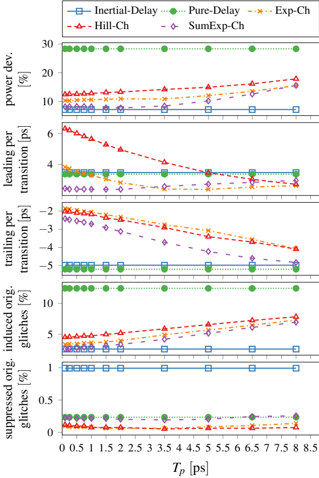
Figure 14: NAND circuit simulation results (65 nm) for \mu = 45 ps, with channels placed at the output.
