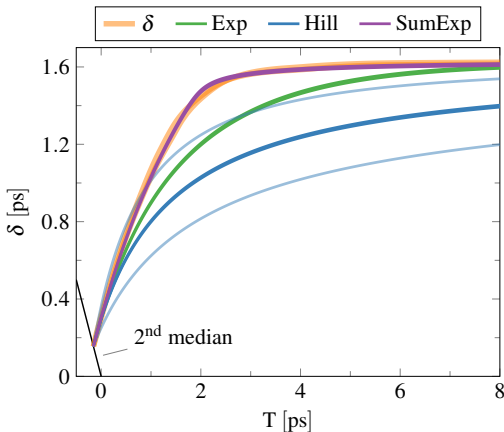
(b) delay function
