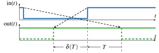
Figure 2: The input pulse is so short that the transitions at the output appear in reverse order (dashed lines), i.e., cancel. Note that here T < 0 and \delta(T) < 0 .
