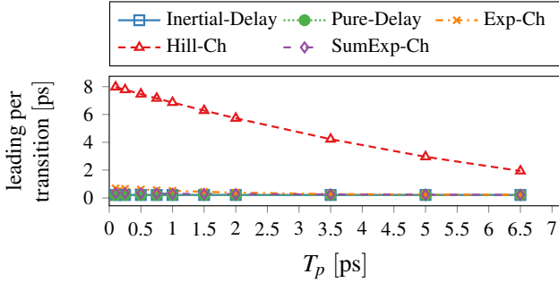
Figure 12: Inverter tree simulation results (65 nm) for \mu = 100 ps.
