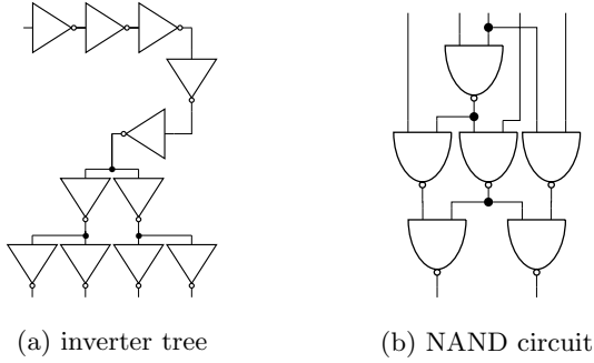
Figure 8: Schematic of circuits used for simulation.
