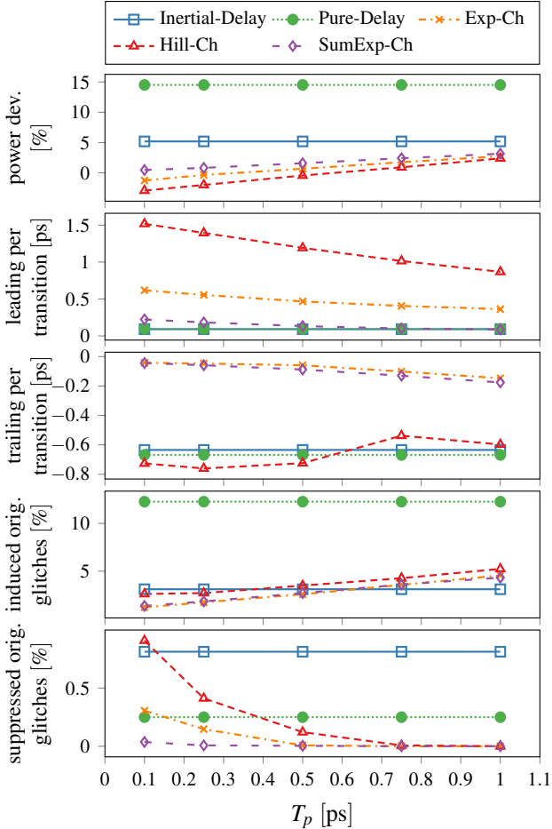
Figure 10: Inverter tree simulation results (15 nm) for \mu = 15 ps.
