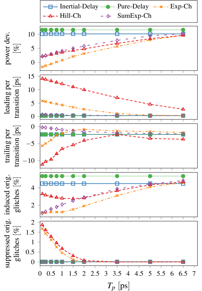
Figure 9: Inverter tree simulation results (65 nm) for \mu = 45 ps.
