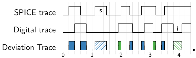
Figure 7: Categorization of the deviation between analog and digital simulation. Shown are pulses (dashed areas) caused by original induced (i) or original suppressed glitches (s) and the leading (blue) and trailing metric (green).
