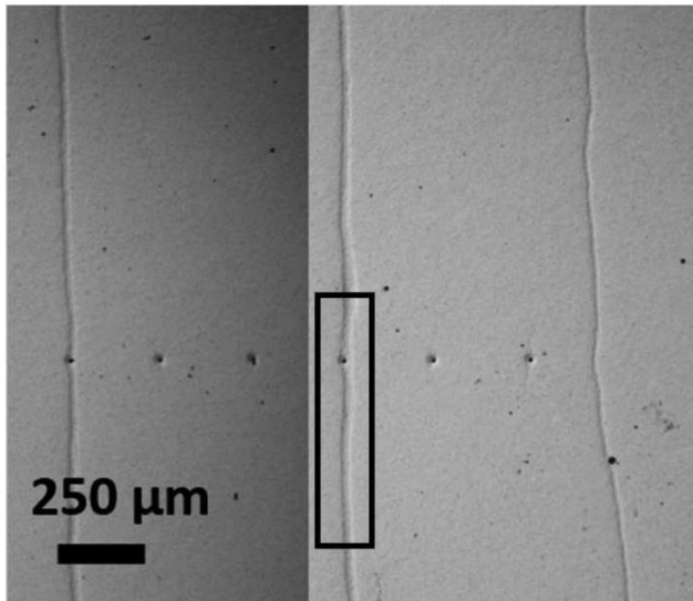
(b) 3 mm thick - 1016 N - break
