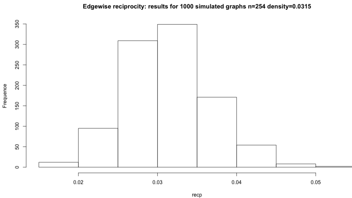
Figure S.I. 2: Simulated reciprocity for 1000 graphs with similar density and number of nodes as our network.
