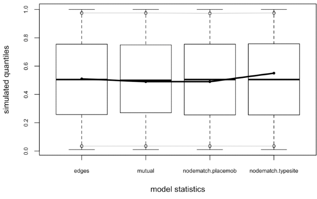
Figure S.I.5 - Goodness of fit and sample statistics for ERGM model 1
