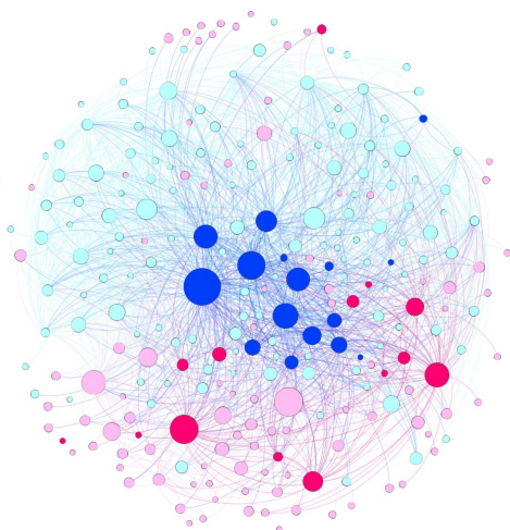
GLOBAL NETWORK SIZE BY VISIBILITY IN THE MEDIA
