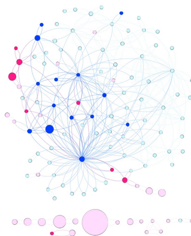
MUTUAL LINKS SIZE BY VISIBILITY IN THE MEDIA
