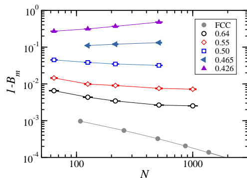
FIG. 12. (Color online) (a) Log-log plots of 1 - B_m vs N for temperature T = 0.175 and the values of \Phi indicated in the Figure. As stressed by the lines connecting the data points, B_m does not saturate to 1 in the thermodynamic limit for any random packing considered, in contrast with the FCC case.
