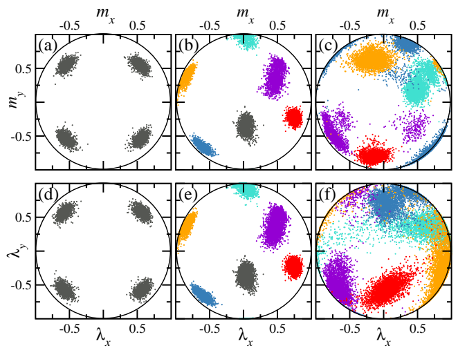
FIG. 5. (Color online) Upper row: thermal distribution of the x - and y -components of the normalized magnetization vector \hat{m} (provided that m_z \geq 0 ). The samples are distinguished by the colors. (a) has been obtained in a FCC lattice; (b) and (c) at \Phi = 0.64 and 0.426 respectively. Lower row: thermal distribution of the nematic director \hat{\lambda} (on the condition that \lambda_z \geq 0 ). (d) stands for the FCC lattice; (e) and (f) for \Phi = 0.64 , and 0.426 respectively. All the distributions are for samples with N = 512 particles at temperature T = 0.1 .
