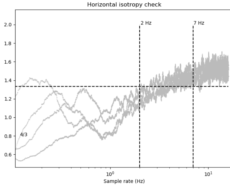
Figure 5. Horizontal isotropy per day of the experiment. The 4/3 theoretical value is denoted by the horizontal dashed line.
