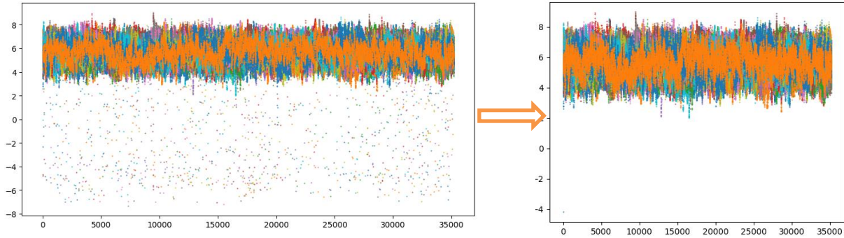
Figure 1. Superimposition of all the 100 second time series of the longitudinal wind component, for the first day of the experiment. The yaw ( \psi ) rotation was applied either at 32 Hz (left panel) or at 1 Hz (right panel). On the left panel, there are outlier points that correspond to wind speed values smaller than 2 m/s. These points did not appear in the original time series (before yaw rotation was applied), which is not shown here. After smoothing at 1 Hz (right panel), the outliers disappear.
