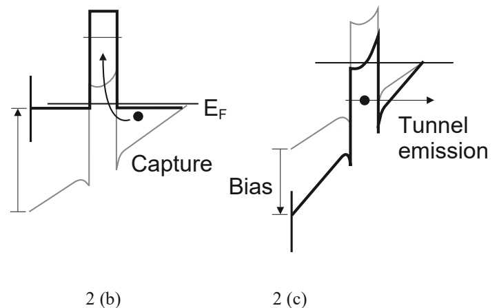
Fig.2: Schematic representation of the valence band during memory operations in QD-Flash: (a) store, (b) write (writing “1”), and (c) erase (writing “0”).
