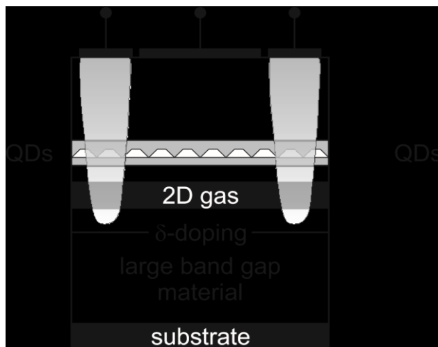
Fig. 1: Sketch of a QD-Flash
