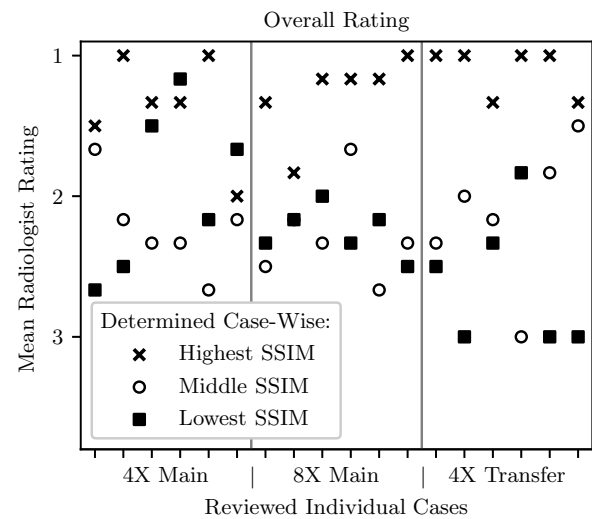
Fig. 5. Scatter plot of mean radiologist rank across cases. The horizontal axis has a separate tick for each case evaluated by the radiologist cohort. The scatter plot markers indicate whether that method was from the team with the highest, middle, or lowest SSIM scores. We generally observed radiologists awarding the best ranks to models with the best SSIM score.
