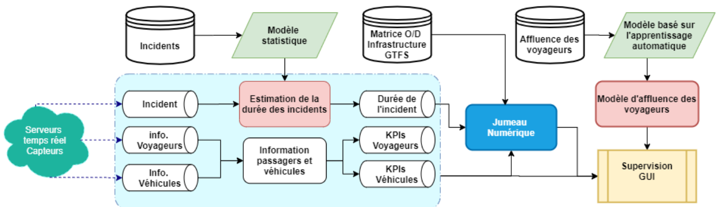
Figure 1 : Architecture générale
