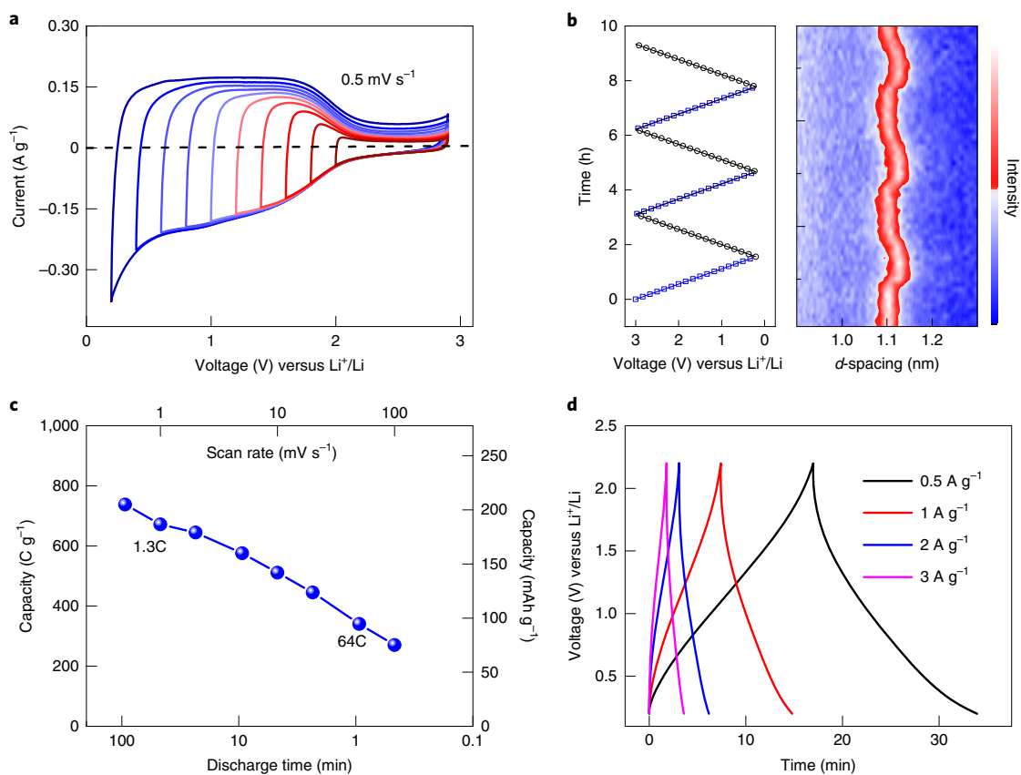
Fig. 4 | Electrochemical characterizations of MS-Ti 3 C 2 T x MXene electrode in 1M LiPF 6 (in 1:1 ethylene carbonate/dimethyl carbonate) electrolyte.
