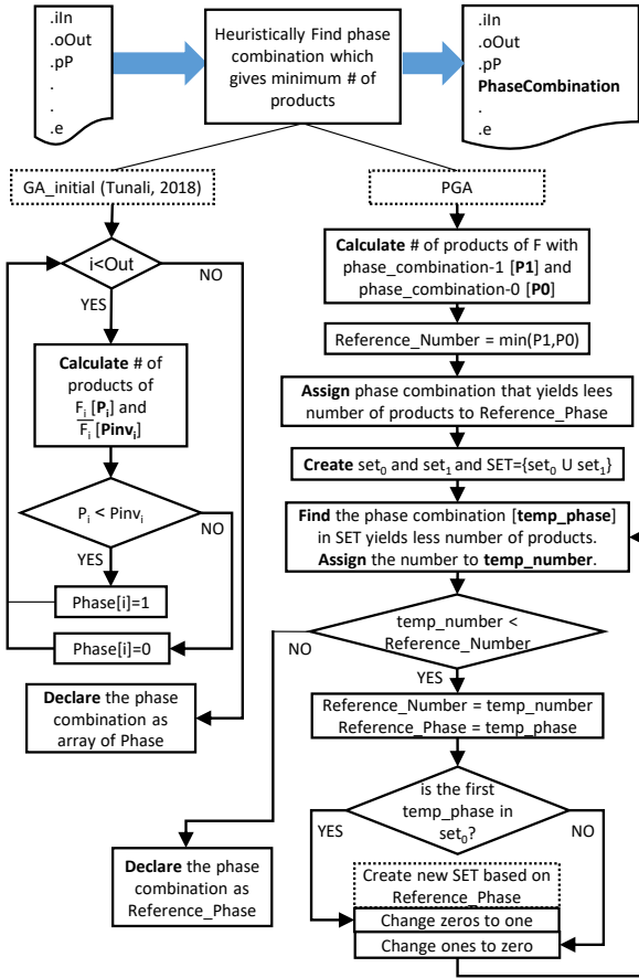
Fig. 4. Block diagrams of two-level multi output logic synthesis algorithms: initial Greedy Algorithm (GA-initial) [43] and Proposed Greedy Algorithm (PGA)
