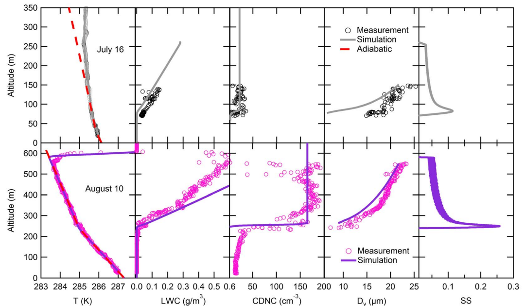
Figure 2. Measured, fitted and simulated profiles of temperature ( T ), liquid water content (LWC), cloud droplet number concentration (CDNC), volume mean diameter ( D_v ), and supersaturation (SS) profiles for the CIRPAS Twin Otter flights and ACP model runs for the 10 August and 16 July cases during E-PEACE. The simulations shown are the EJL16B-sa and EAG10B-ad cases from Table 1. For comparison, the adiabatic lapse rate is also shown as a red dashed line. The observations did not include cloud top for 16 July.
