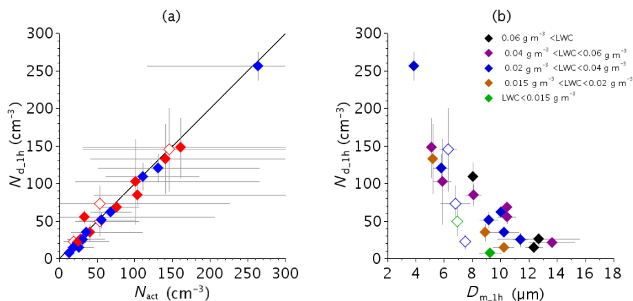
Figure 12. Droplet number concentration at the beginning of the fog for the 23 cases as a function of (a) the activated particle concentration ( N_{act} ) and (b) the mean fog diameter. Diamonds correspond to median values and error bars to 25th–75th percentile intervals. Symbol colors are as a function of (a) fog type as in Fig. 2 and (b) LWC values as indicated in the legend.
