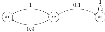
Figure 1: An example of DTMC \mathcal{M}_1
