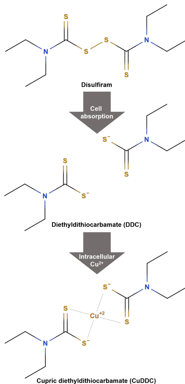
Fig. 1. Disulfiram (DSF) reaction with copper. The DSF's disulfide bond (S-S) is promptly reduced after cell intake thus producing diethylthiocarbamate (DDC), which is a strong chelator of transition divalent metal ions, such as copper (II).
