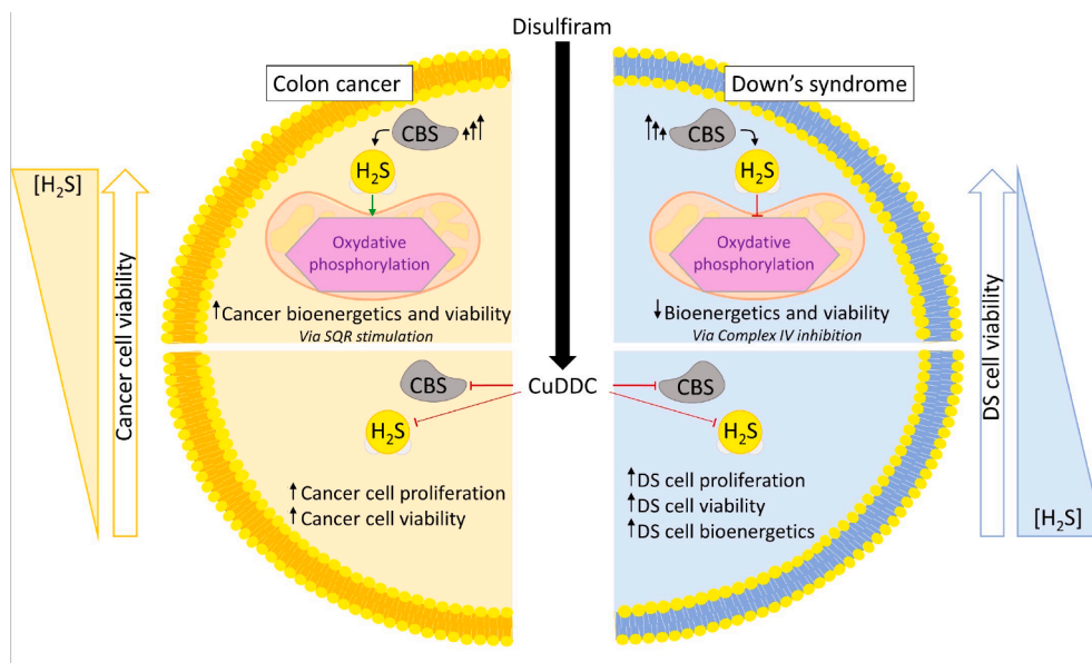
Fig. 10. Effect of disulfiram and its metabolite CuDDC on the H_2S system in cancer and Down's syndrome cell models. In colon cancer cells, the excess of H_2S supports cellular bioenergetics. Here, sulfide:quinone oxidoreductase (SQR) couples sulfide detoxification with energy production. Vice versa , in fibroblasts, where the sulfide oxidizing system is less represented, an increment H_2S levels may result in mitochondrial impairment because of cytochrome c oxidase (CcOX) inhibition. Disulfiram, through its metabolite CuDDC lowers intracellular H_2S levels through inhibition of cystathionine \beta -synthase and direct H_2S scavenging. This results in reduction or increase of cell viability and proliferation in colon cancer and DS fibroblasts, respectively. Disulfiram, through its metabolite CuDDC, lowers intracellular H_2S levels through inhibition of its biosynthesis, thus resulting in decrease or increase of cell viability in cancer and Down's syndrome fibroblasts, respectively.
