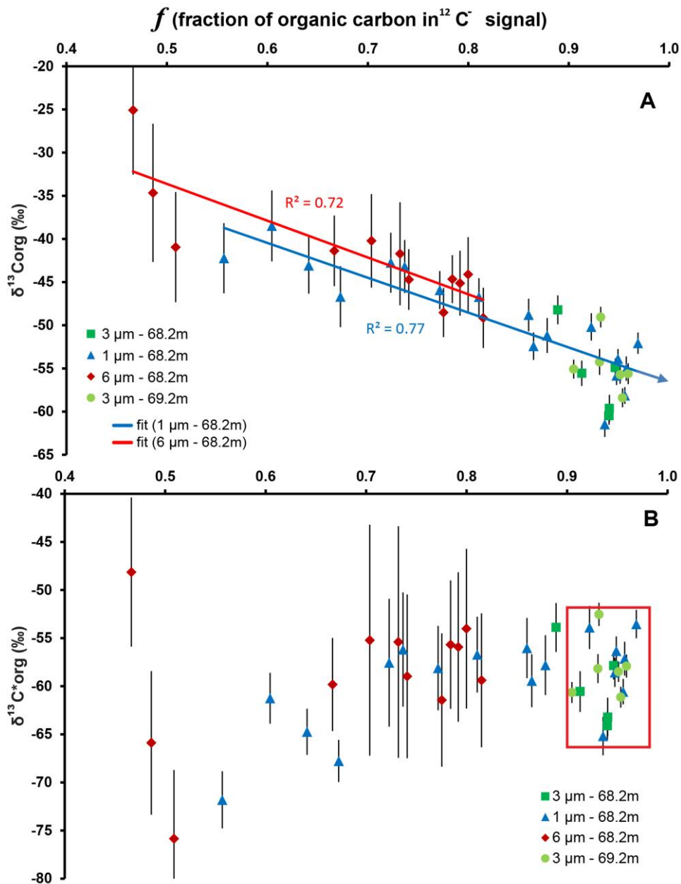
Fig. 10. SIMS analyses of micrometric Type-B organic globules in calcite crystals recorded with SIMS spot size of 1, 3 and 6 \mu\text{m} . (A) Plot of \delta^{13}\text{C}_{\text{org}} (2SE error bars) against f (the fraction of organic C in total ^{12}\text{C}^- signal, see equation 10) values. The analytical sessions with 1- and 6- \mu\text{m} spots display a wide range of f where \delta^{13}\text{C}_{\text{org}} decreases with increasing f , indicating that at low OM concentrations (low f ), the signal contains a mixture of carbonate and organic carbons (see text). (B) Mass balance calculation (using equations 11–15) provide \delta^{13}\text{C}^*\text{org} values (2SE* error bars) corrected of interference of carbonate. The red box indicates the values that satisfy the filtering criterion f > 0.9 (see text).
