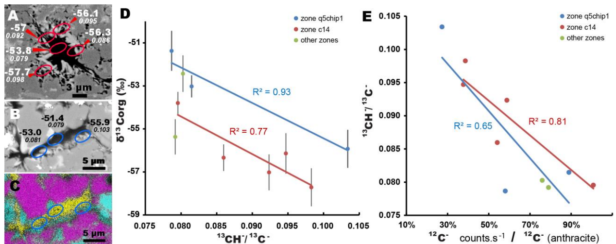
Fig. 8 SIMS analyses (3- \mu\text{m} spot) of Type-A organic matter in contact with chlorite \pm quartz. (A-B) SEM BSE images of zones q5chip1 (A) and c14 (B) of sample KGI68.2'. SIMS targets (circled in A-C) were chosen in order to sample zones with variable OM (in black) to chlorite (light grey to white) \pm quartz (medium grey) concentrations ratios. (C) SEM-EDXS map of Si (pink, from quartz and chlorite), Al (cyan, from chlorite), and C (yellow, from OM) in the zone of (B). (D) The ^{13}\text{CH}^-/^{13}\text{C}^- ratios display large variations compared to those recorded in quartz as shown in Fig. 7. Linear
