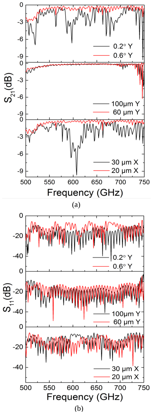
Fig. 8. Simulated insertion losses for different misaligned position of taper at 1 mm inside MWG a) S 21 parameter (transmittance) b) S 11 parameter (Reflectance)
