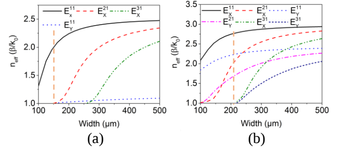
Fig. 1 Normalized propagation constant at 650 GHz as function of waveguide width (W) for a) thickness T=50 \mu\text{m} and b) T=90 \mu\text{m} .
