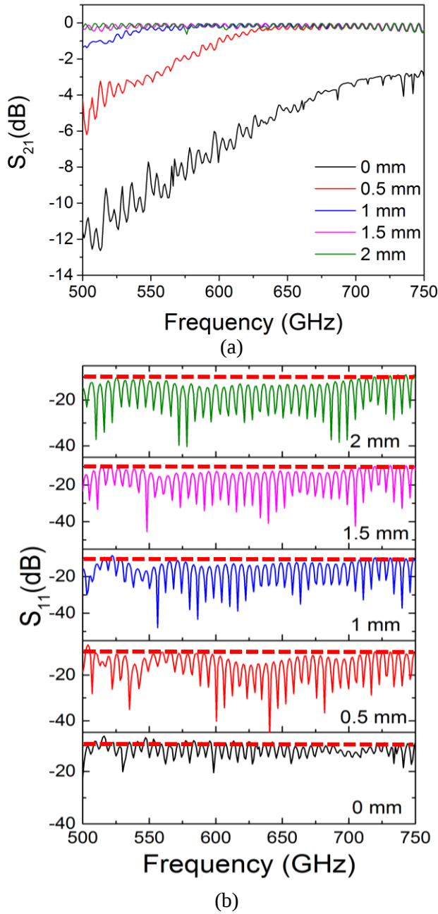
Fig. 7. Simulated insertion losses for different position of taper inside MWG with the red dashed horizontal line indicating the 10 dB level a) S 21 parameter (transmittance) b) S 11 parameter (Reflectance)
