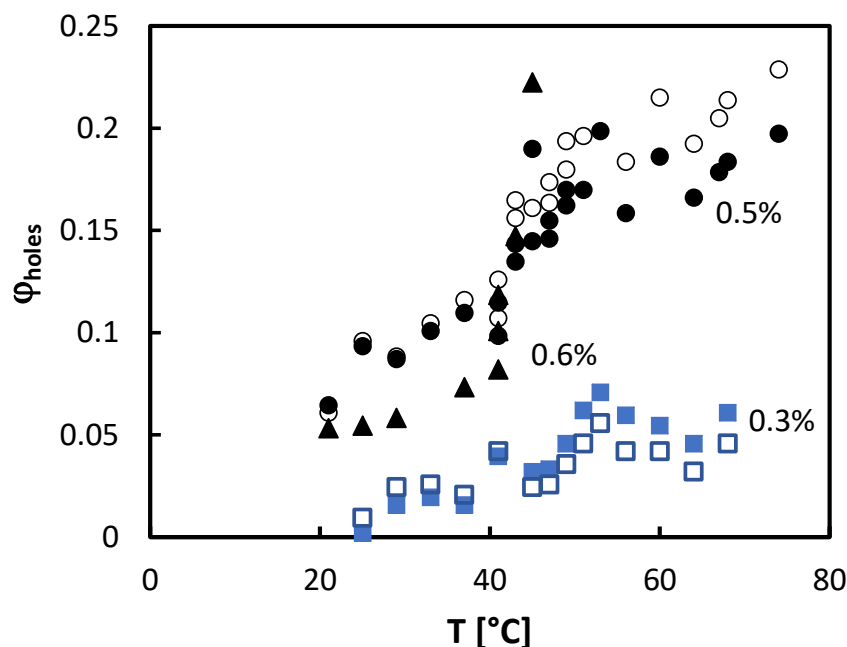
Figure 8: Surface fraction of holes ( \phi_{hole} ) containing D 2 O vs. temperature for films in contact with BA/PTR2/D 2 O for BA fraction of 0.3%, 0.5% and 0.6%. \phi_{hole} was deduced from fitting the NR spectra to a crossing hole model (full symbols) and non-crossing holes (empty symbols).
