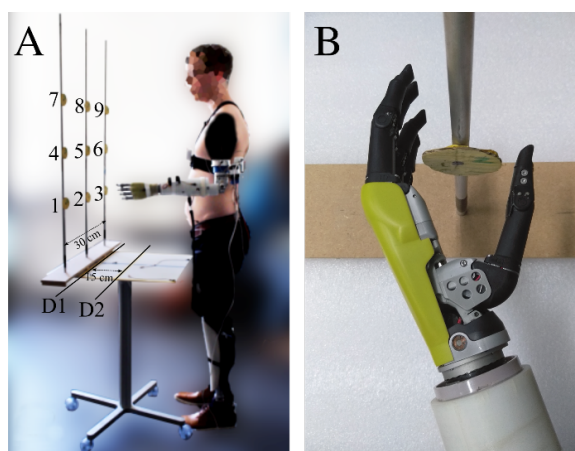
Figure 1: Experimental setup. A: amputated participant wearing the prototype and standing in the initial position. 9 targets are shown for each distance (D1 and D2). B: Hand position with respect to the target when successfully reaching a target.
