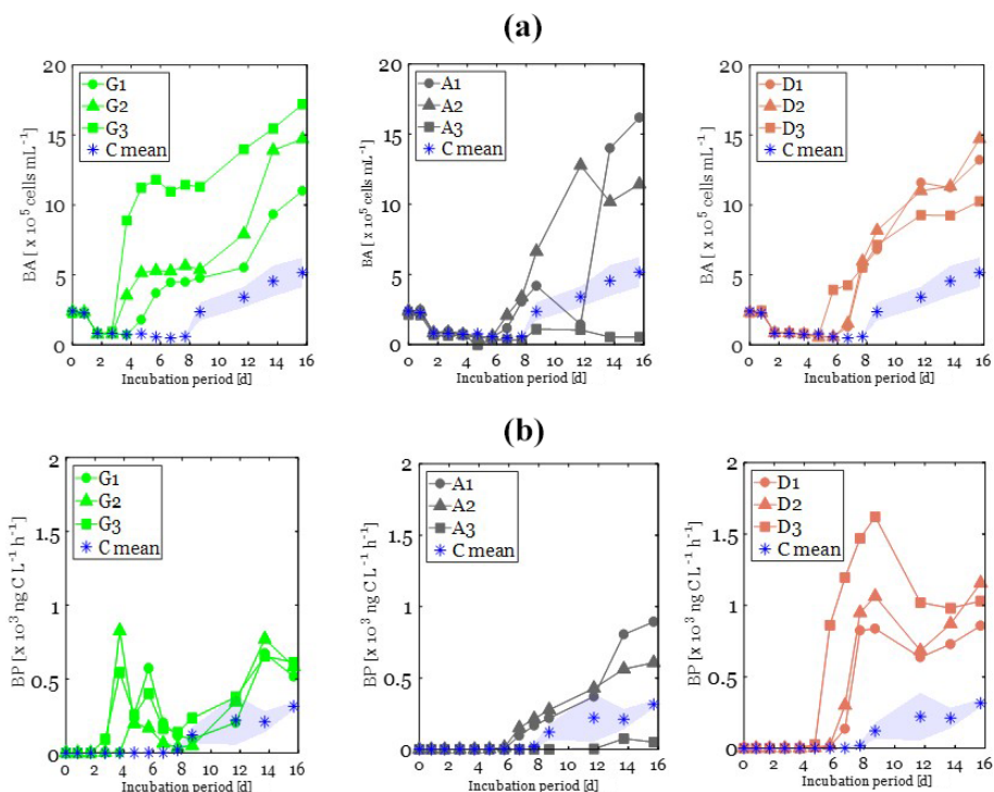
Figure 3. Changes in heterotrophic bacterial abundance (BA; a ) and production (BP, b ) over the incubation period in glucose (left, green plots), anthropogenic aerosols (middle, gray plots), and Saharan dust aerosols (right, orange plots). The control is plotted in each panel: the average value is represented by the stars and the standard deviation by the bounded lines.
