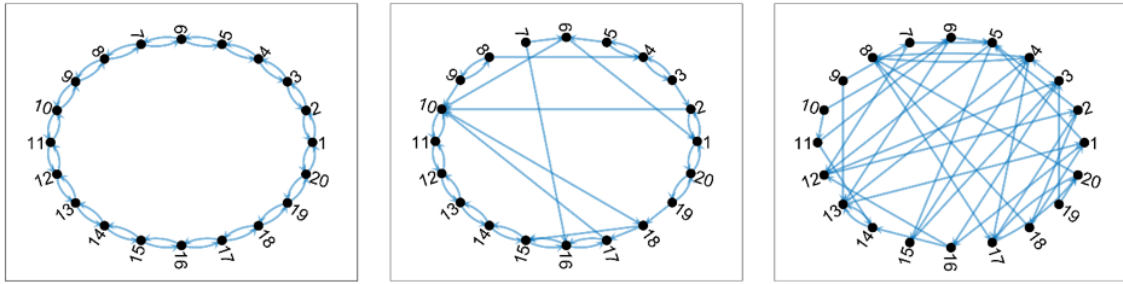
Figure 11. Example of the creation of a small-world network.
