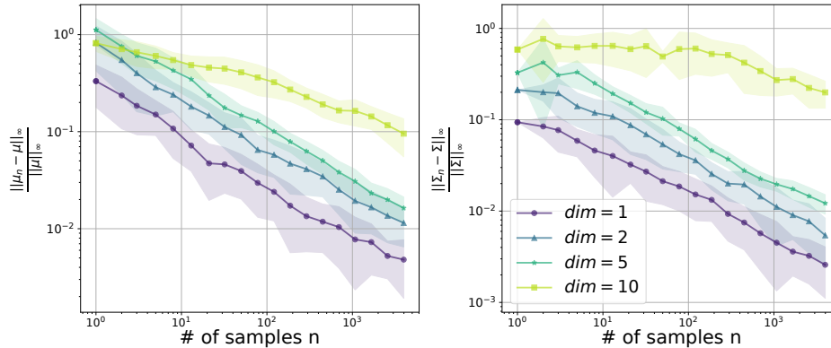
Figure 3: Numerical convergence the (n -samples) empirical estimation of the theoretical mean \mu and covariance \mathbf{H} of theorem 3. Empirical moments are computed computed using Sinkhorn’s algorithm.
