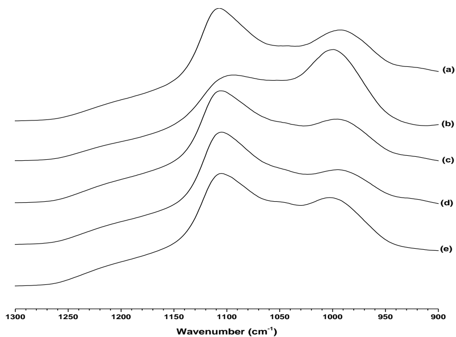
Fig. Erreur ! Document principal seulement. FTIR spectra of modified gels with (a) KOH, (b) NaOH, (c) AlOOH, (d) \text{Li}_2\text{B}_4\text{O}_7 and (e) HCl in the interval 1300-900 \text{cm}^{-1} at 20 °C after 1h under stirring
