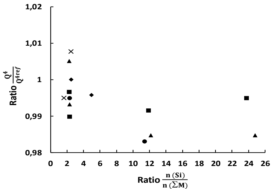
Fig. 4 Values of the ratio \frac{Q^4}{Q^{4ref}} as a function of the ratio \frac{n(\text{Si})}{n(\Sigma\text{M})} of the silica mixtures with (◆)KOH, (●)NaOH, (■) AlOOH, (▲) \text{Li}_2\text{B}_4\text{O}_7 and (×) HCl
