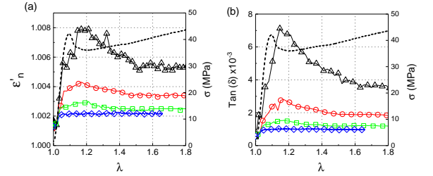
FIG. 3. Normalized real part \varepsilon'_n (a) and \tan\delta (b) as a function of \lambda measured at 7Hz for different strain rates : 2.5 \times 10^{-3} \text{ s}^{-1} (black triangles), 2.5 \times 10^{-4} \text{ s}^{-1} (red circles), 2.5 \times 10^{-5} \text{ s}^{-1} (green squares) and 2.5 \times 10^{-6} \text{ s}^{-1} (blue diamonds).
