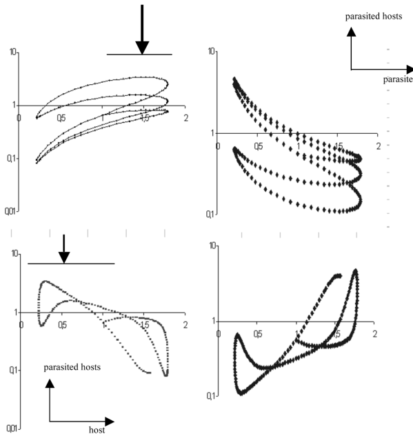
FIG. 3 : Ratio Parasite/Host : Hypothesis for modelling : non overlappig cohorts, delay between successive cohorts is longer for the parasite, (Left) or for the host (Right). Estimated maximal parasitism rate (in each cohort, % of parasited females depends on parasite densities). Two factors are tested: the density of host (bottom) or density of potential parasites. (Ratio between the H and P periods is 1/3 in both cases). Aggregate distribution is expected when number of parasites is high and hosts are rarer (Left, arrow) when parasite's development is the longest. Maximal values of the ratio parasite/host depends on host number when host's development is longer (Right).
