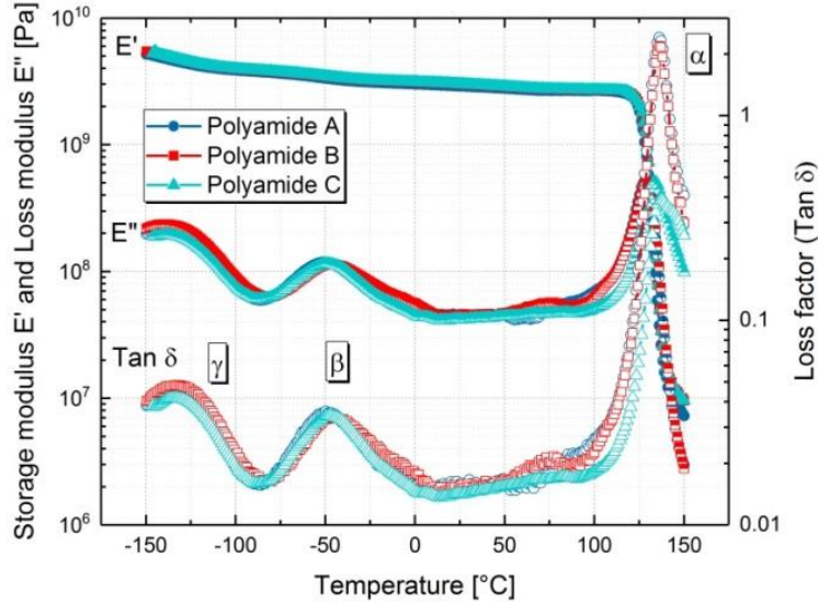
Figure 4 Temperature dependences of the storage modulus E' , the loss modulus E'' and the damping factor \tan\delta , as determined at 1 Hz for the different PPA by DMTA measurements. The different relaxation processes are indicated on the \tan\delta curves.
