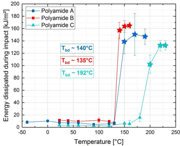
Figure 6 Brittle-ductile transition curves of all the PPA samples obtained from Charpy impact measurements. Evolution of the energy dissipated by the material with the temperature and the brittle-ductile transition temperature T_{bd} . The stars represent the unbroken samples above the T_{bd} .
