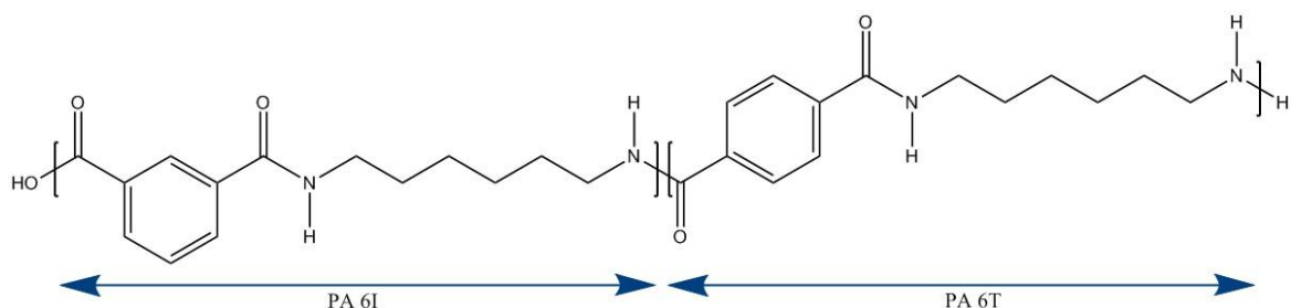
Figure 1 Structure of the copolymer PA6I/6T.
