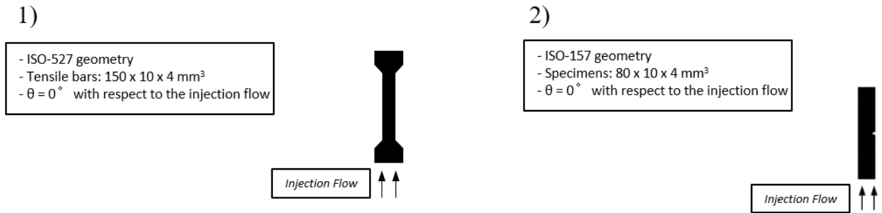
Figure 2 Tensile and impact geometries of the specimens.
