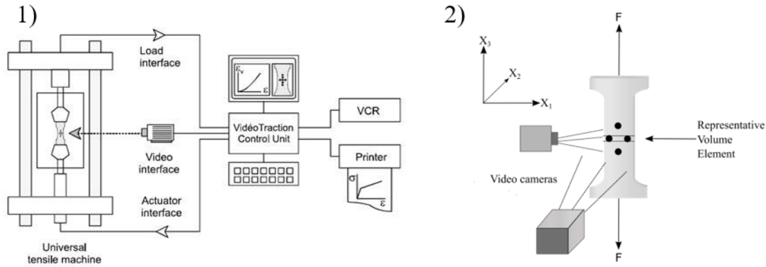
Figure 3 Representation of the VidéoTraction® system (1) and the markers on the middle of the tensile specimen with the two cameras (2). Adapted from [23] with permission from Elsevier.
