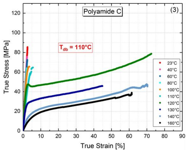
Figure 7 Uniaxial tensile true stress-true strain curves determined for Polyamide A (1), Polyamide B (2) and Polyamide C (3) at several temperatures and a strain rate of 1 \cdot 10^{-3} \text{ s}^{-1} .
