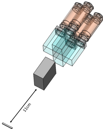
Figure 3: The drawing of the cross-shaped detector assembly is shown in the top of the figure. The four PWO crystals are mounted along the four sides of a tungsten block. Each PWO crystal is assembled with cylindrical PMT. The target cavity drawn as a thin box is at the bottom of figure. The tungsten block is installed between the detector assembly and the target cavity.
