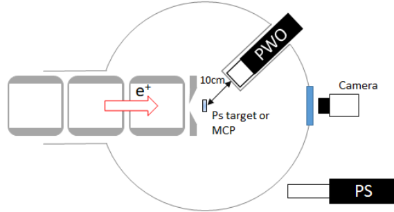
Figure 1: Schematic view of the target area. The tubes with gray color show the Einzel lenses for the positron beam focusing. The circular line outlines the reaction chamber. The positronium converter and the MCP assembly are translated by a linear drive to place them at the center of the chamber. A camera is placed downstream of the MCP assembly to image the positron beam profile. The PWO detector and a plastic scintillator (PS) are installed at the backside of the target region for the \gamma ray measurement.
