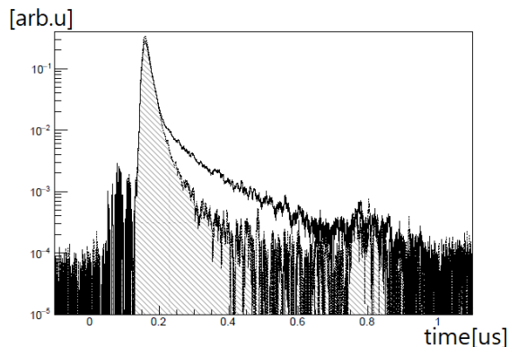
Figure 2: The raw signal distribution from the PWO detector (averaged data sample). The diagonal filled histogram shows the signal from the PWO detector when the e^+ beam hits the MCP and the solid line histogram shows the signal when the e^+ beam hits the positronium converter.
