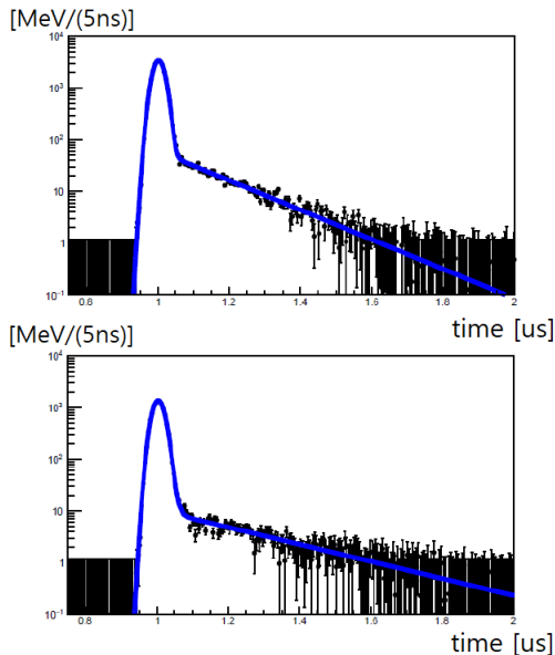
Figure 4: The simulated raw signal distribution of the detector assembly. The positron pulse is simulated by a Gaussian distribution and the angular distribution at emission or reflection of o-Ps is isotropic. The raw signal distributions at the left and right PWO detectors (top panel) and the top and bottom PWO detectors (bottom panel) are shown. The solid line shows the fitted PDF.
