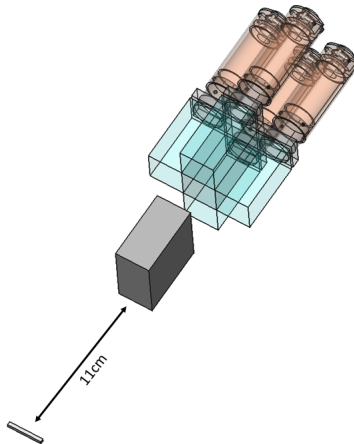
Figure 3: The drawing of the cross-shaped detector assembly is shown in the top of the figure. The four PWO crystals are mounted along the four sides of a tungsten block. Each PWO crystal is assembled with cylindrical PMT. The target cavity drawn as a thin box is at the bottom of figure. The tungsten block is installed between the detector assembly and the target cavity.
