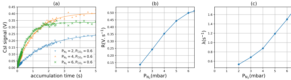
Figure 2: (a) Number of e^+ as measured by the CsI detector, fit with N(t) + c . (b) R vs N_2 pressure. (c) Positron annihilation rate ( \lambda = 1/\tau ) vs N_2 pressure. Pressures in mbar as measured at the injection point of the system.
