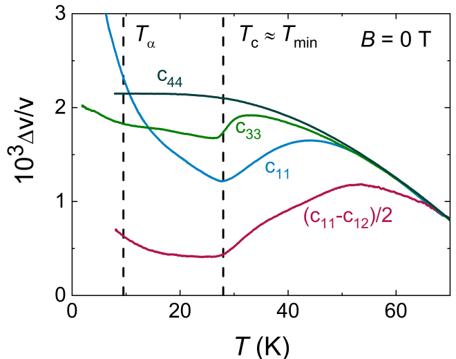
Figure 1: Sound velocity variation, \Delta v/v , as a function of temperature for different acoustic modes as indicated. No magnetic field is applied, the curves are arbitrarily superimposed at T=70 K. T_{\min} refers to the minimum in the c_{11} elastic constant that coincides with the superconducting T_c in zero magnetic field. T_\alpha indicates the spin freezing temperature at the \mu\text{eV} ultrasound energy scale, defined by an attenuation peak (see Fig. 2).
