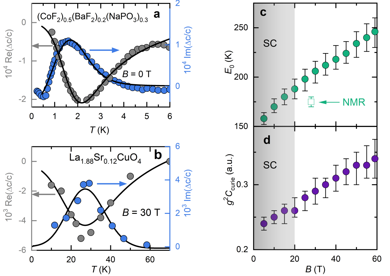
Figure 5: Fitting of the experimental \Re(\Delta c/c) (gray circles, left scale) and \Im(\Delta c/c) (blue circles, right scale) for (a) the cobalt fluorophosphate canonical spin glass in a longitudinal acoustic mode reproduced from Ref.[28] and (b) LSCO p = 0.12 at B = 30 T in the (c_{11} - c_{12})/2 transverse mode. In panels (a) and (b) a background sound velocity has been subtracted. The black lines are fit to the data using the dynamical susceptibility model. Fitting parameters for cobalt fluorophosphate are E_0 \approx 18 K and g^2 C_{\text{curie}} \approx 10^{-3} a.u.. Fitting parameters for LSCO p = 0.12 are shown in panels (c) E_0 and (d) g^2 C_{\text{curie}} . The other two free parameters, g^2 \chi_0 \approx -4.5 a.u. and \Delta E_0 \approx 70 K, don't show any significant field dependence. For comparison E_0 extracted from NMR 1/T_1 at 28 T found in Fig. 4 (empty square) is also shown. The error bars on a single parameter are estimated by monitoring the error of the fit with all other parameters fixed.
