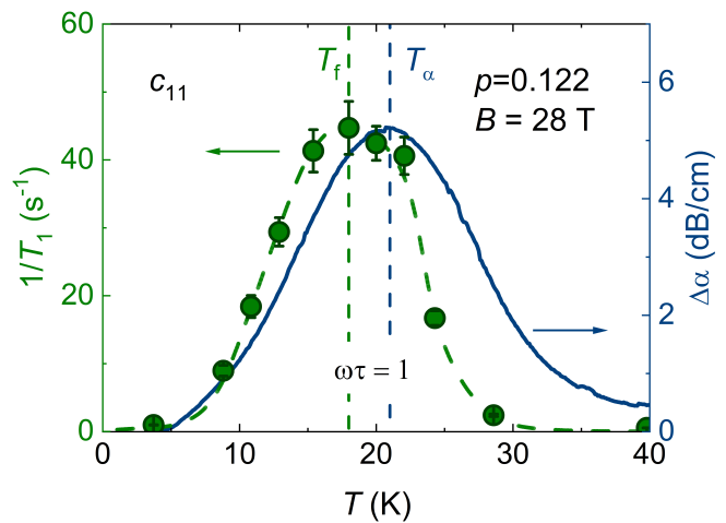
Figure 4: Comparison between the ultrasound attenuation \Delta\alpha (blue line, right scale) and the ^{139}\text{La} NMR spin-lattice relaxation rate 1/T_1 (green circle, left scale), at B = 28 T. NMR and ultrasound samples are from the same batch. Both physical quantities show a peak when the excitation frequency becomes equal to the frequency of the spin fluctuations, i.e. \omega\tau = 1 . A phenomenological linear background has been subtracted from the experimental \Delta\alpha for clarity. The dashed green line is a guide to the eye.
