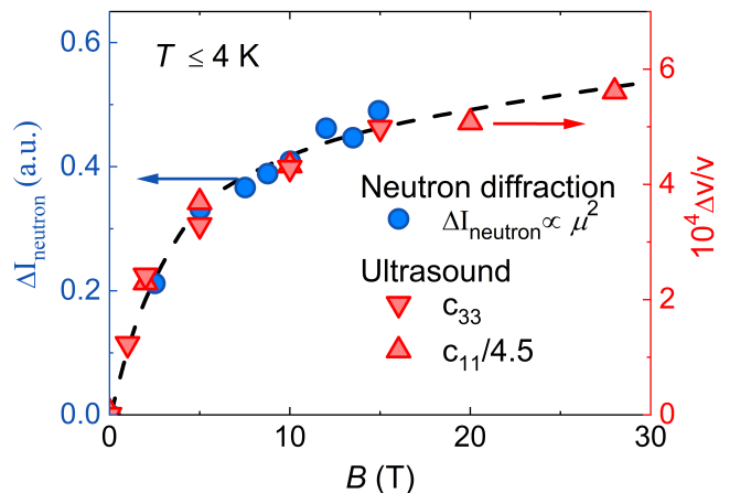
Figure 7: Comparison between the magnetic field dependence of the superlattice Bragg peak intensity of incommensurate AFM seen by neutron diffraction, \Delta I_{\text{neutron}} (blue circles, left scale), and the sound velocity, \Delta v/v , in the c_{11} and c_{33} acoustic modes (up and down red triangles respectively, right scale). The neutron diffraction intensity is reproduced from Ref. [42]. The sound velocity in the c_{11} mode is divided by a factor 4.5. The sound velocity measurements presented here are taken at T \leq 4 K in field-cooled conditions. The dashed line is a guide to the eye.
