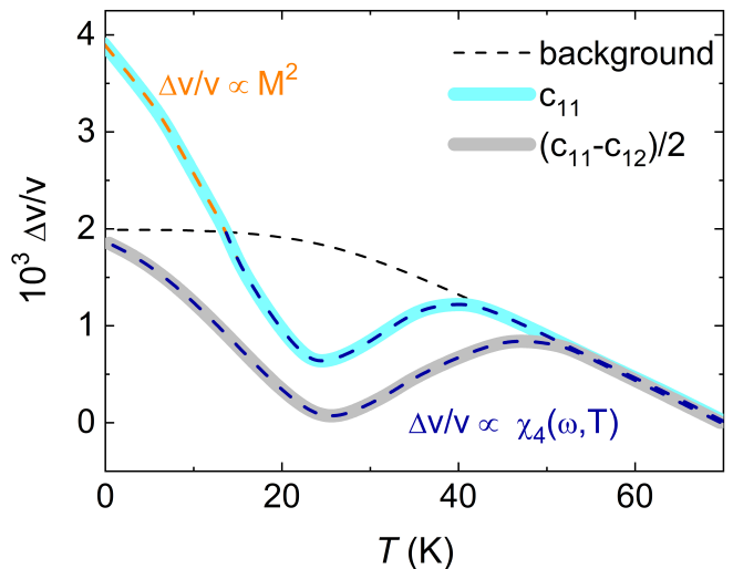
Figure 6: Schematic representation of the sound velocity of the (c_{11} - c_{12})/2 (grey) and c_{11} (cyan) modes in LSCO p = 0.12 . Black dashed line is the background elastic constant arising from anharmonicity of ionic potential [20]. (c_{11} - c_{12})/2 can be fully reproduced by the dynamical susceptibility model involving \chi_4(\omega, T) (dashed blue line). For T \rightarrow 0 , the difference between the sound velocity of the (c_{11} - c_{12})/2 mode and its background tends to zero. This contrasts with the behaviour of c_{11} . For T \rightarrow 0 , the sound velocity of the c_{11} mode is larger than the background sound velocity. This means that in addition to the contribution from \chi_4(\omega, T) (dashed blue line) that causes the minimum in c_{11} , another component contributes at low T . As discussed in the text, a contribution proportional to M^2 (dashed orange line) could explain the rapid increase of c_{11} at low temperature.
