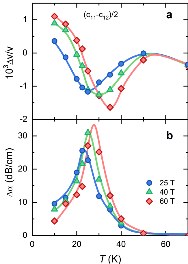
Figure 3: Temperature dependence of the (c_{11} - c_{12})/2 acoustic mode in pulsed-fields up to 60 T. (a) \Delta v/v and (b) \Delta\alpha both extracted from fixed magnetic field cuts of the pulsed-fields isotherms to which we add the zero field curve. All lines are guides to the eye.
