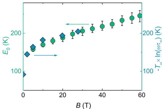
Figure B.1: Comparison between the E_0 energy scale (circles, left scale) extracted from the fitting procedure of Fig. 5 and -T_\alpha \times \ln(\omega\tau_\infty) (diamonds, right scale) determined directly from the data shown in Fig. 2(b), \omega = 2\pi \times 110 MHz and \tau_\infty \approx 10^{-13} s. The energy scale -T_\alpha \times \ln(\omega\tau_\infty) corresponds to an experimental determination of E_0 solely based on T_\alpha , using the condition \omega\tau_4(T_\alpha) = 1 in Eq. 6 (see text). The rapid drop of -T_\alpha \times \ln(\omega\tau_\infty) at low B is most likely due to the impact of superconductivity on the spin dynamics. Error bars on this quantity are smaller than the size of the symbols.
