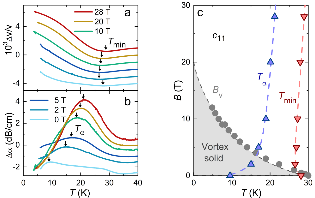
Figure 2: Static field ultrasound measurements in the c_{11} acoustic mode up to 28 T. (a) \Delta v/v and (b) \Delta\alpha as a function of temperature for different magnetic fields. The curves are shifted for clarity. The arrows denote T_{\min} and T_\alpha as indicated. (c) B-T phase diagram: gray circles denote the vortex melting transition field B_v , inferred from in-plane resistivity measurements, T_\alpha (upward-pointing blue triangles) and T_{\min} (downward-pointing red triangles) refer to the maximum in attenuation and minimum in velocity respectively. Error bars are smaller than the symbol size. Dashed lines are guides to the eye.
