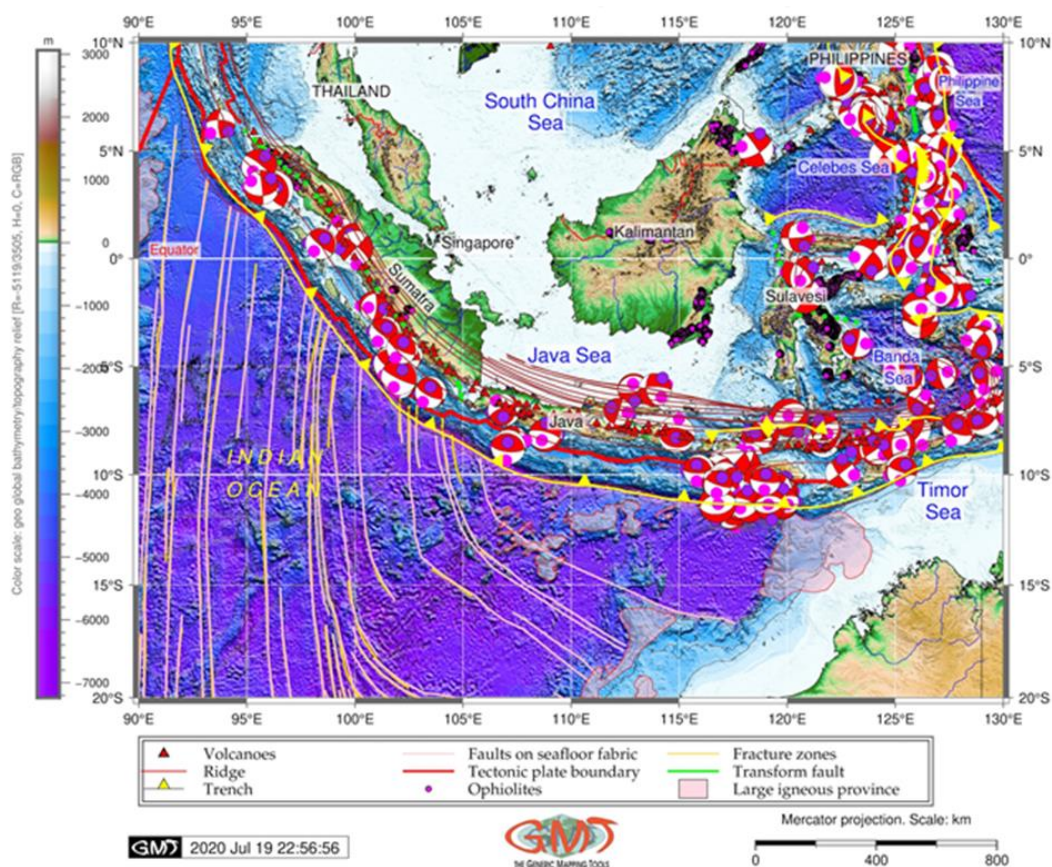
Figure 2 Geologic map of the West Indonesia basin. GEMCO 15 arc sec resolution global terrain model grid
