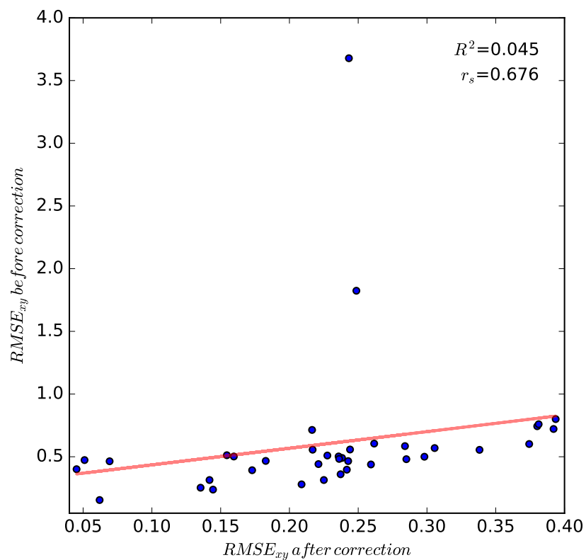
Figure 7. Relationship between the RMSE_{xy} before and after correction for the time-series (31TGG, master 23 August 2016). Due to two outliers the relationship is characterized by a low Pearson's R^2 but shows a monotonic behaviour indicated by a high Spearman rank correlation r_s .
