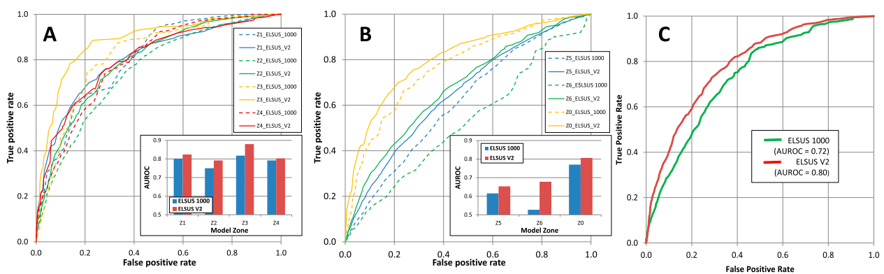
Figure 2. ROC curves and AU ROC values (insets in A and B) detailing the predictive model performance of ELSUS V2 compared to ELSUS 1000 using the updated landslide inventory. (A) Results for ‘plain’; (B) Results for ‘mountainous/coastal’ model zones; (C) Overall prediction model performance of the composite ELSUS 1000 and ELSUS V2 maps.
