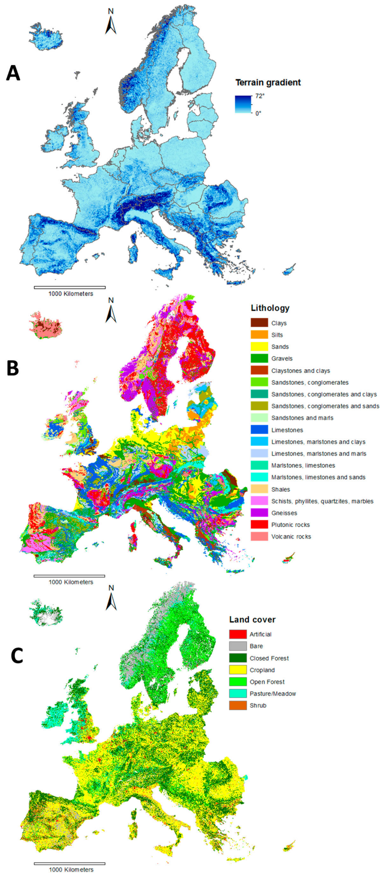
Figure 1. Thematic information used for ELSUS V2. (A) Terrain gradient from EU27 DEM; (B) Lithology from IHME; (C) Land cover from GlobCover.
